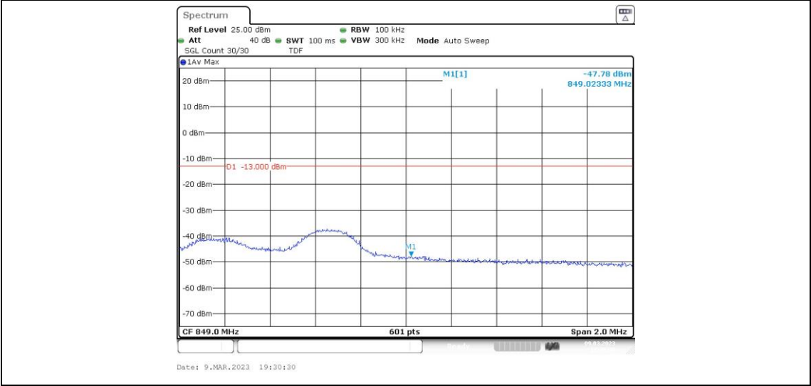
Band26-5MHz-QPSK-27015-1RB#24
