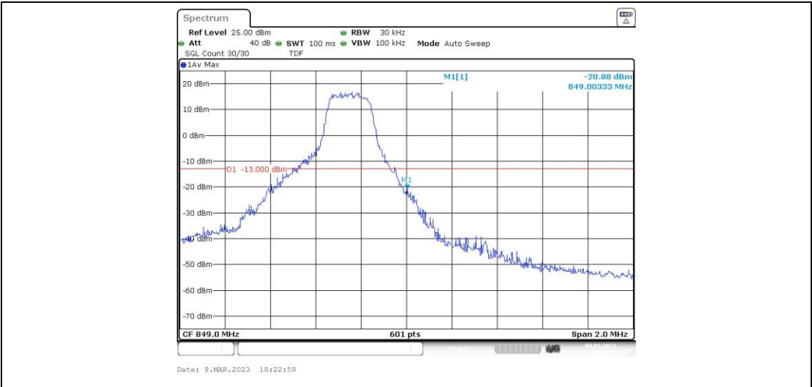
Band26-1.4MHz-QPSK-27033-6RB#0
