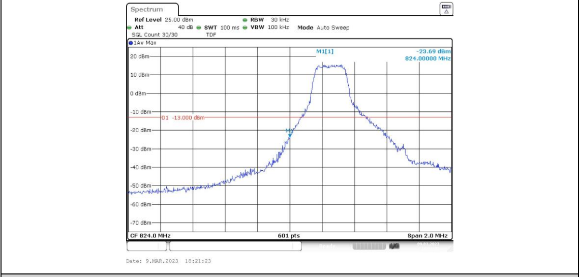
Band26-1.4MHz-16QAM-26797-1RB#5
