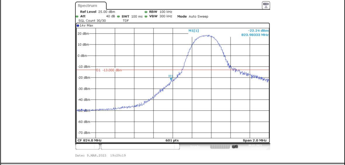
Band26-5MHz-16QAM-26815-1RB#24
