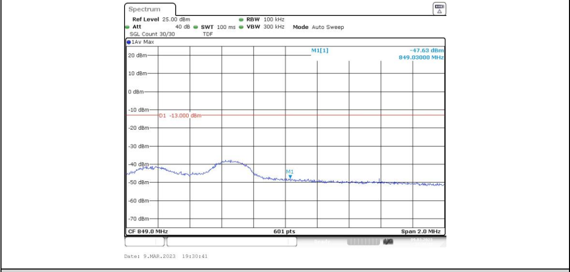
Band26-5MHz-16QAM-27015-1RB#24
