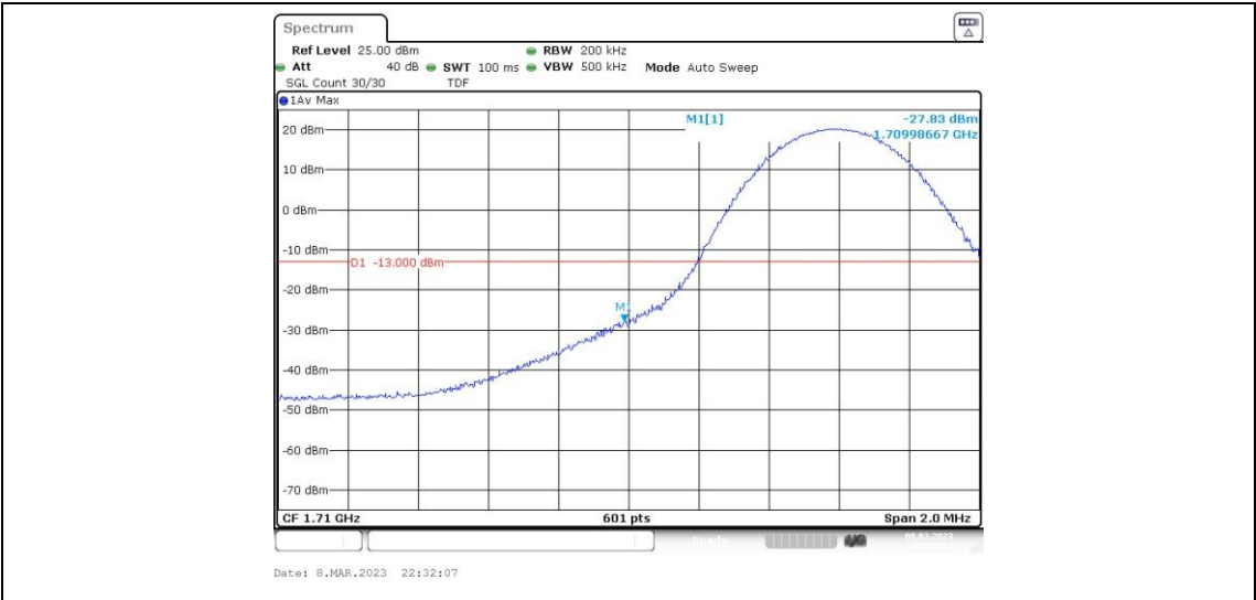
Band4-10MHz-QPSK-20000-1RB#49
