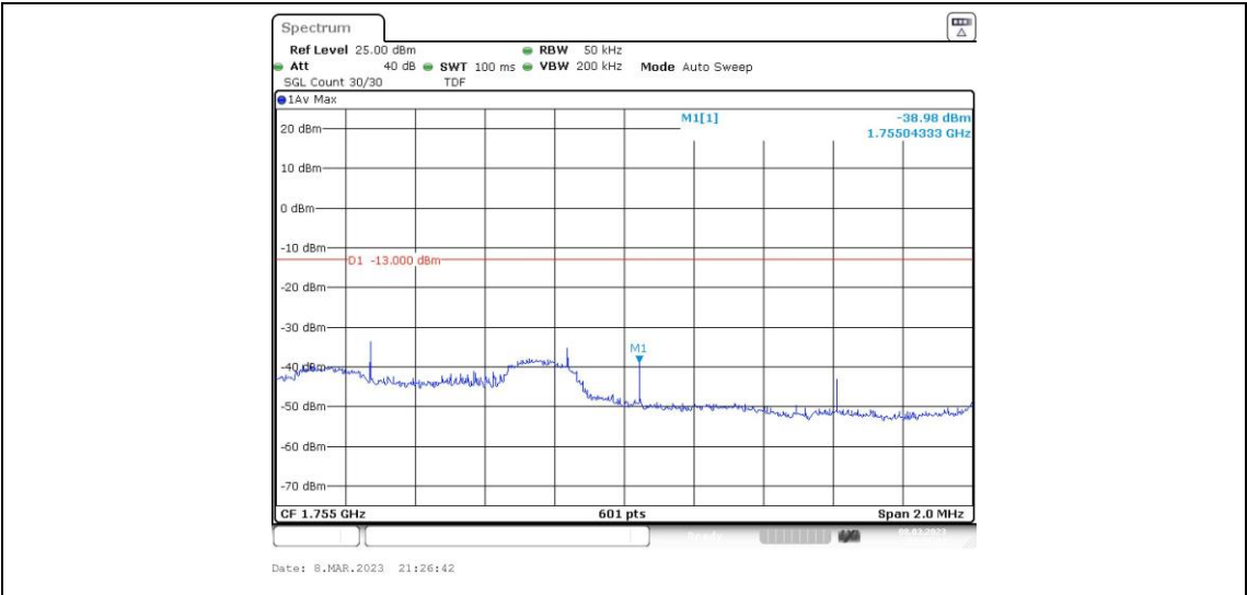
Band4-3MHz-QPSK-20385-1RB#14
