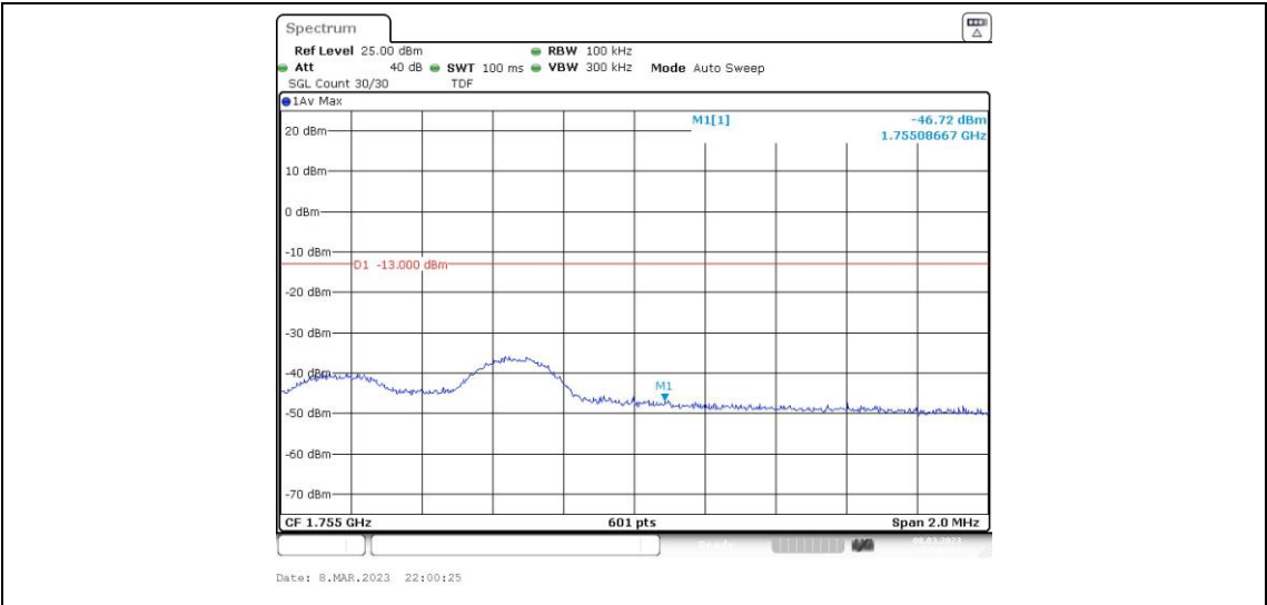
Band4-5MHz-QPSK-20375-1RB#24
