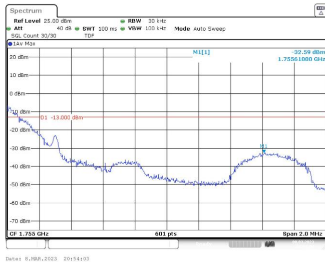
Band4-1.4MHz-QPSK-20393-1RB#5
