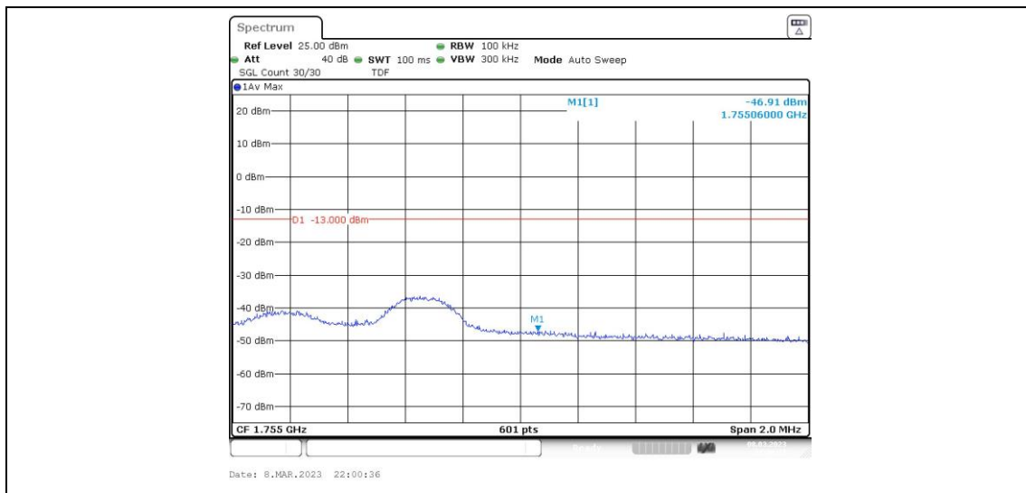
Band4-5MHz-16QAM-20375-1RB#24
