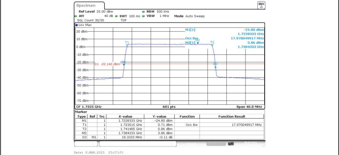
Band4-20MHz-16QAM-20300-100RB#0
