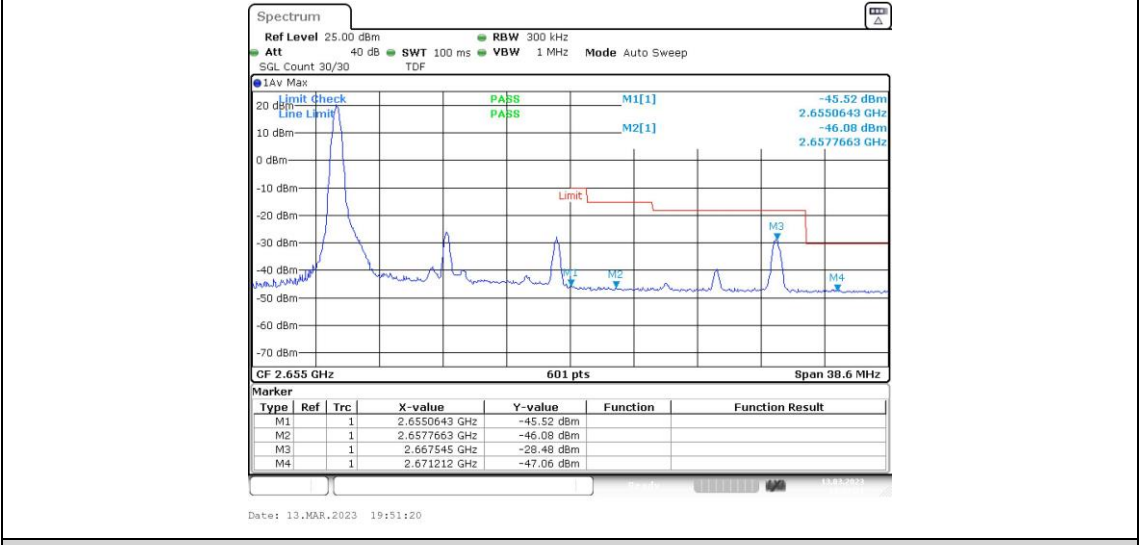
Band41-15MHz-16QAM-41165-1RB#74
