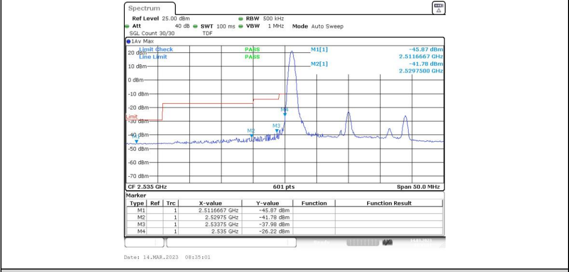
Band41-20MHz-16QAM-40140-1RB#99
