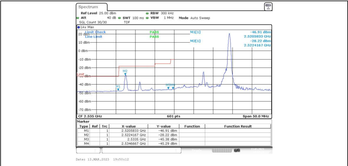
Band41-15MHz-16QAM-40115-75RB#0
