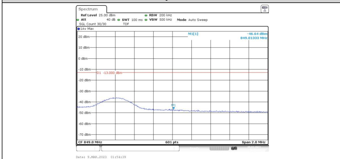
Band5-10MHz-QPSK-20600-1RB#49
