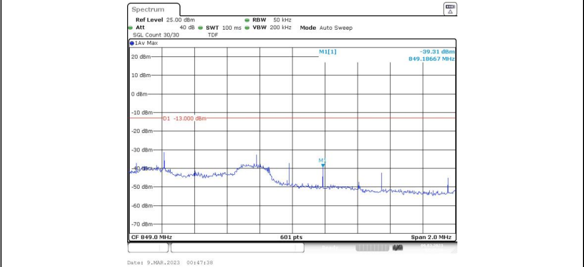
Band5-3MHz-16QAM-20635-1RB#14
