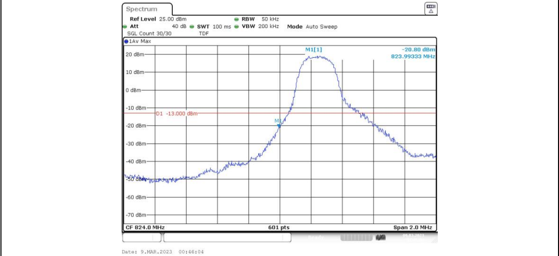
Band5-3MHz-QPSK-20415-1RB#14
