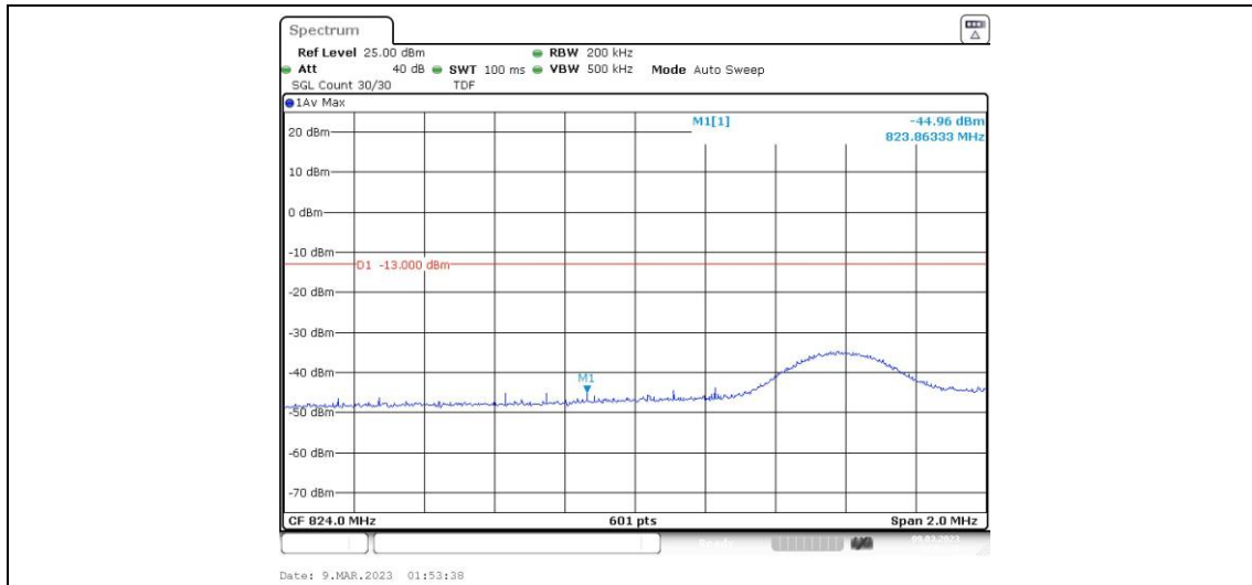
Band5-10MHz-QPSK-20450-50RB#0
