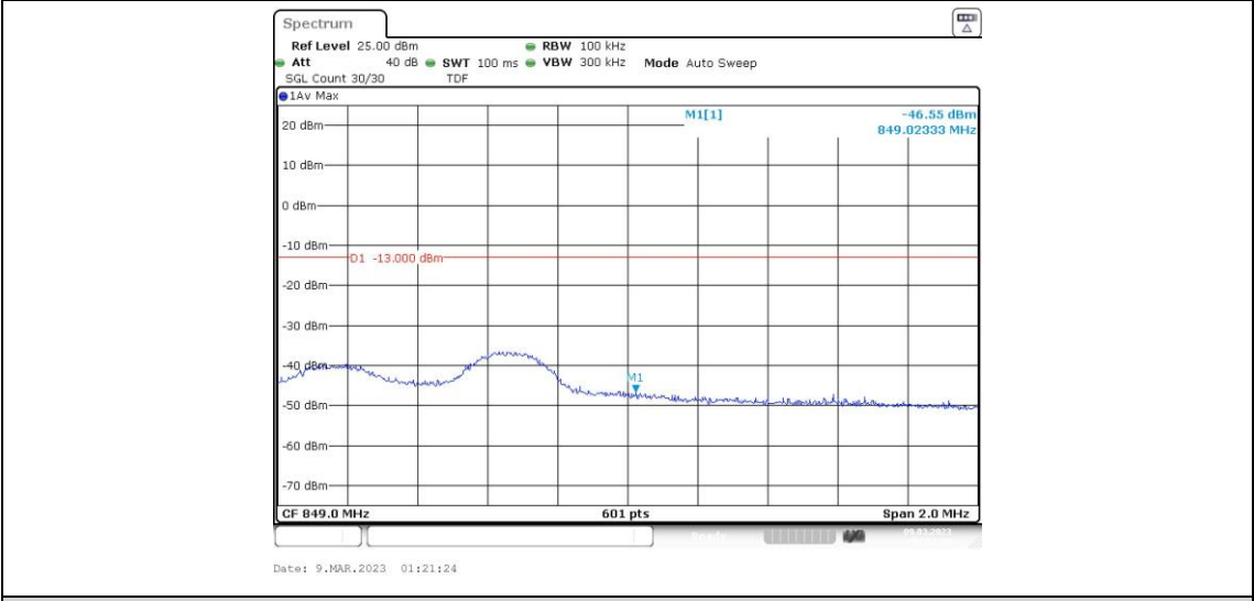
Band5-5MHz-QPSK-20625-1RB#24
