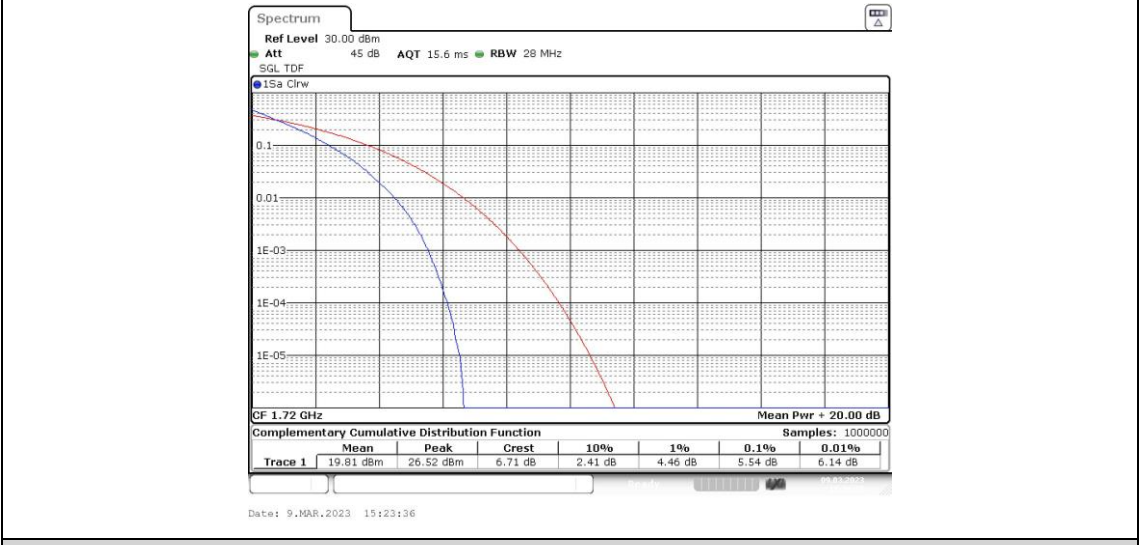
Band66-20MHz-QPSK-132322-1RB#0
