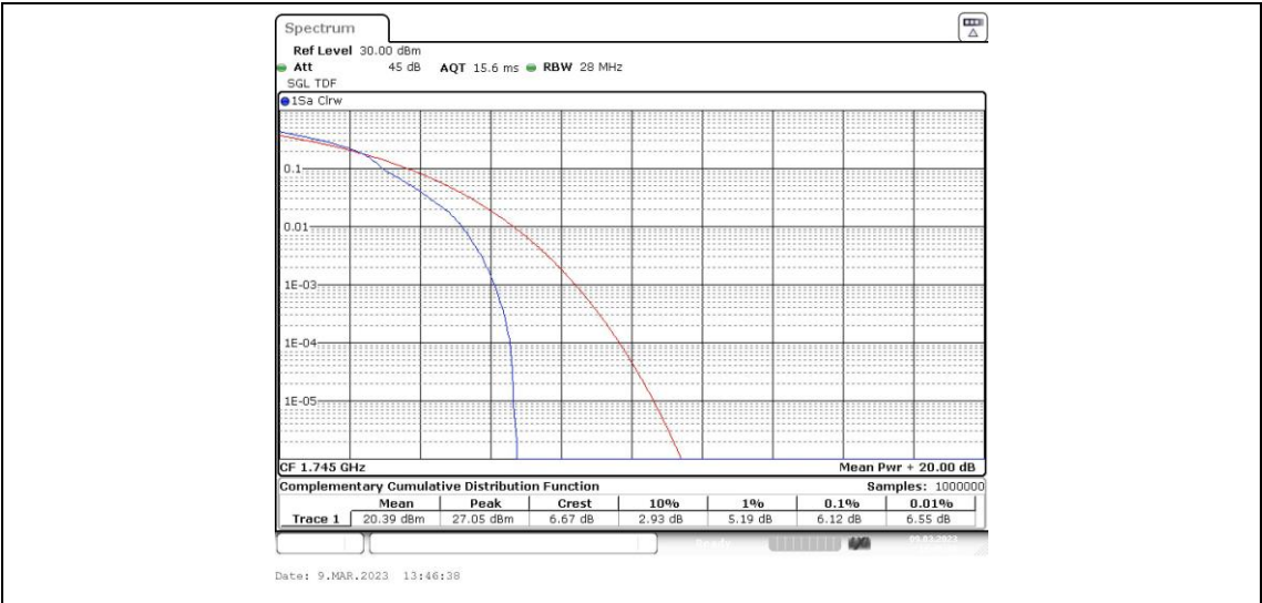
Band66-5MHz-16QAM-132322-25RB#0
