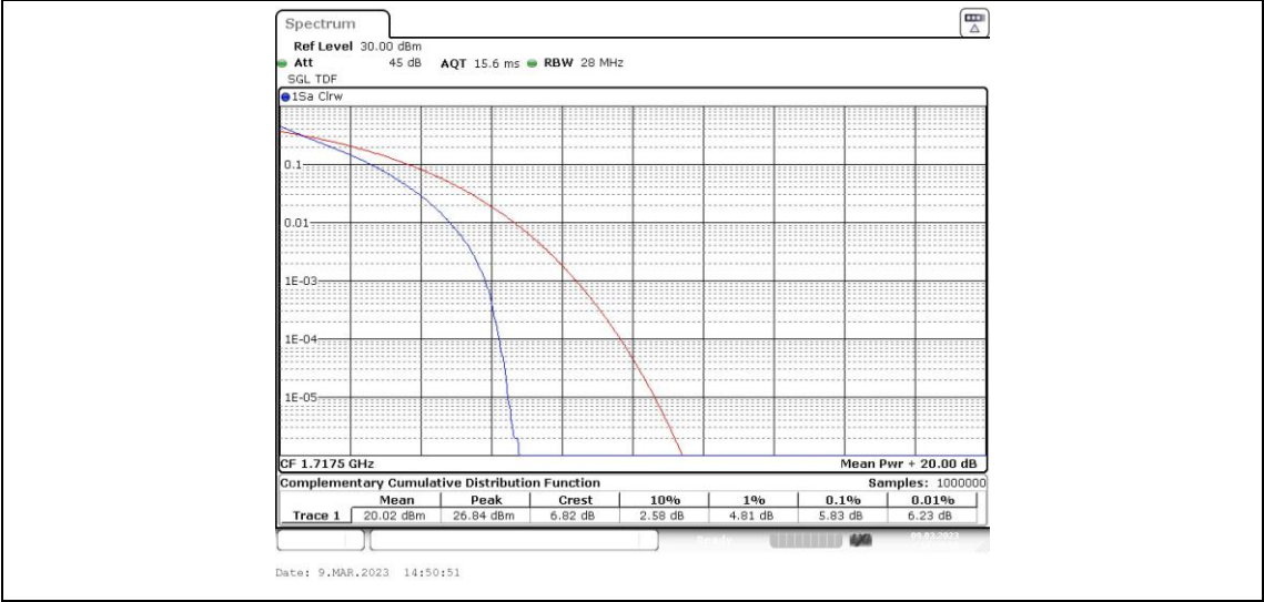
Band66-15MHz-QPSK-132322-1RB#0
