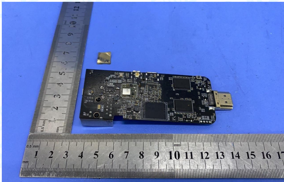
Photo 14 Appearance of Antenna
