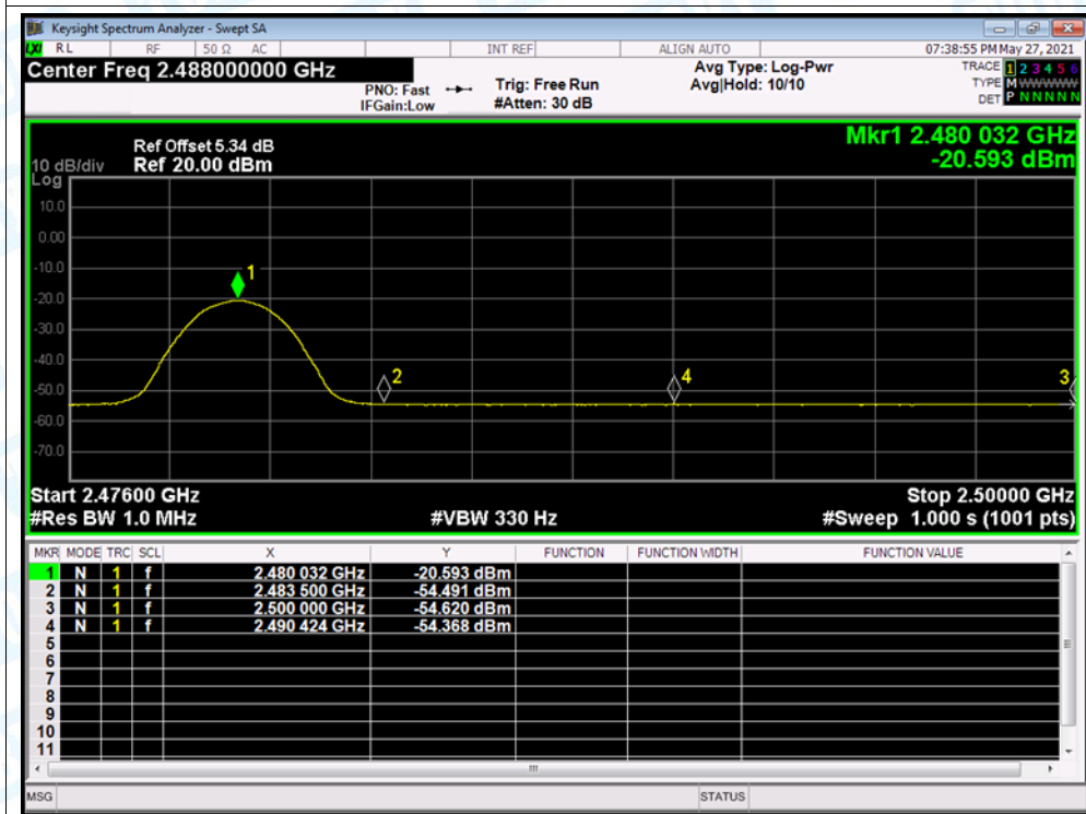
Restrict Band NVNT 2-DH1 2480MHz Ant1 No-Hopping Average
