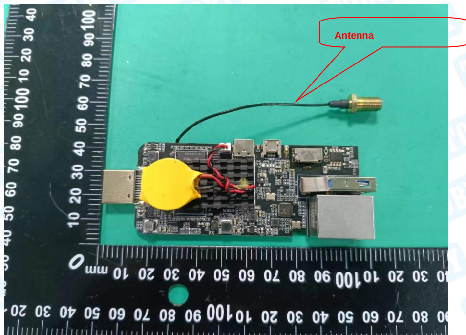
Photo 8 Appearance of PCB
