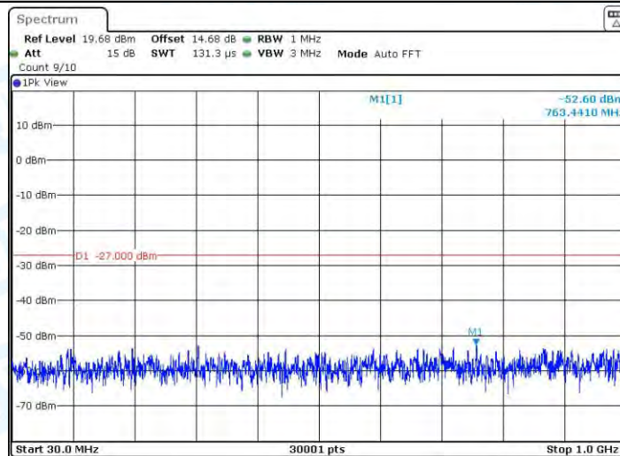
11AC20SISO_Ant1_5240_30~1000
