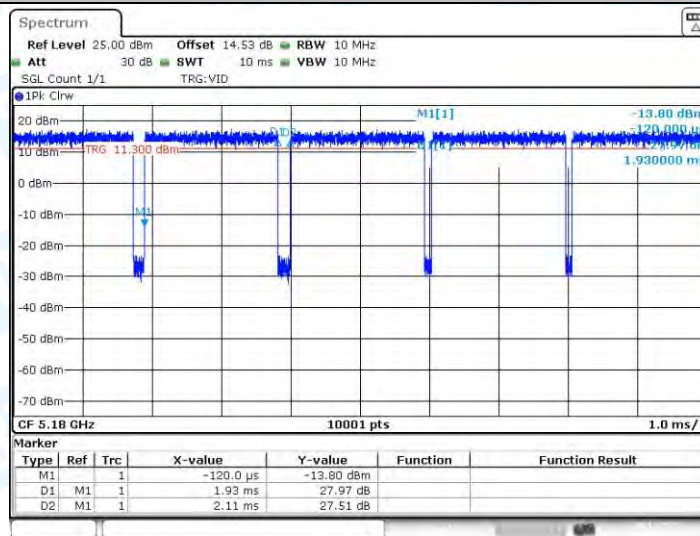
11AC20SISO_Ant1_5180
