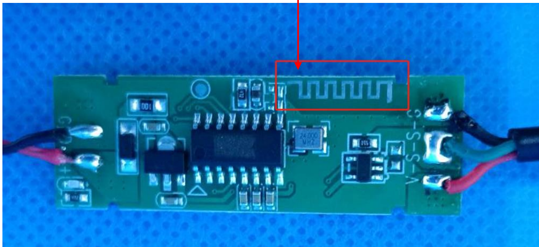
View of wireless antenna
