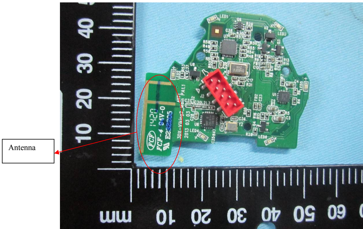
Space Mouse Pro Wireless Mainboard - Front View
