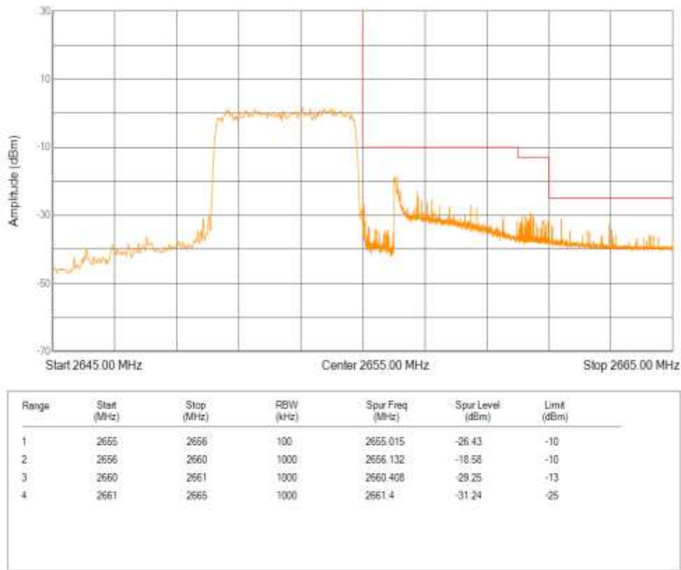
Band41(2655-2665) QPSK BW=10MHz Channel=40290 RB Size=50 Position=#0
