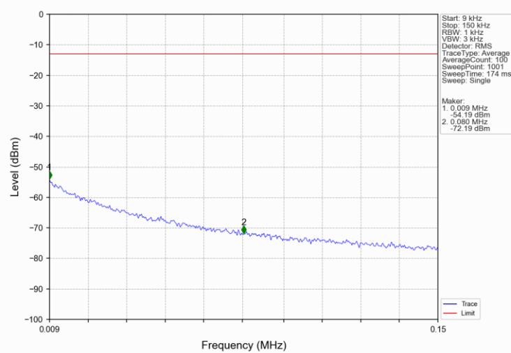
Band12_5MHz_QPSK_LCH_701.5MHz_RB_1_0_NTNV
