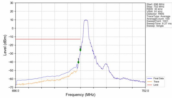
Band12_1.4MHz_QPSK_LCH_699.7MHz_RB_1_0_NTNV
