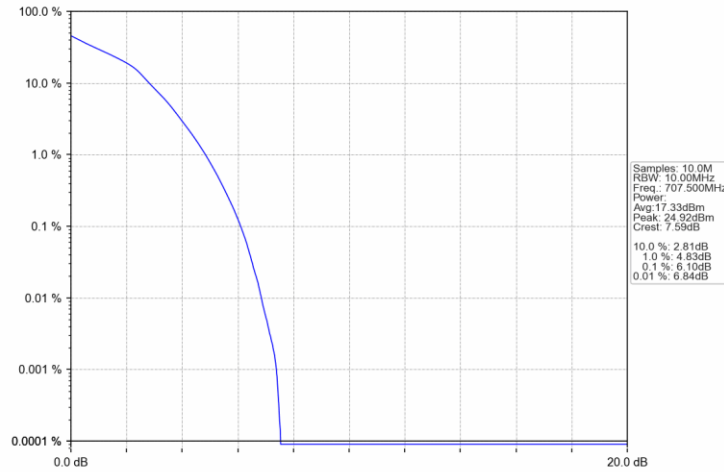
Band12_10MHz_16QAM_MCH_707.5MHz_RB_50_0_NTNV
