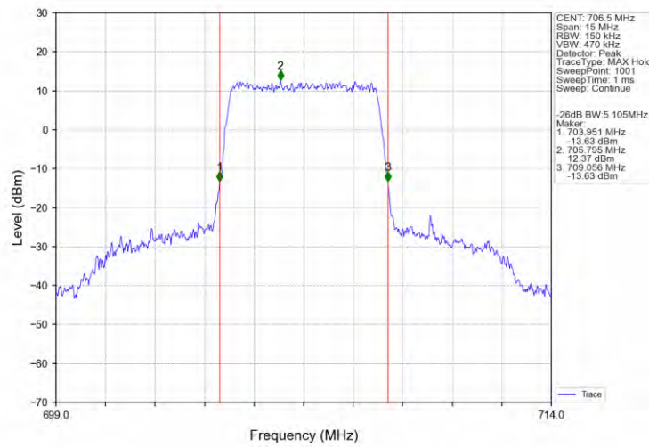
Band17_5MHz_16QAM_LCH_706.5MHz_RB_25_0_NTNV
