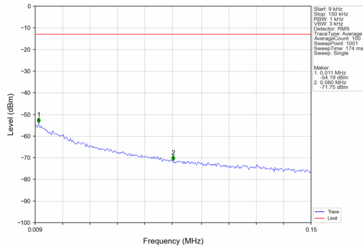
Band25_1.4MHz_16QAM_LCH_1850.7MHz_RB_1_0_NTNV
