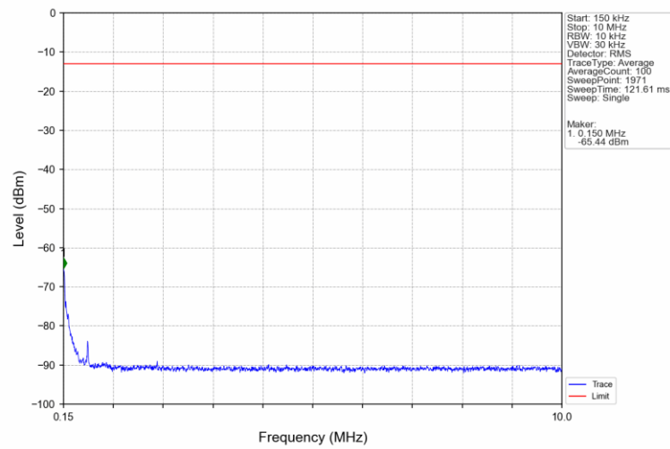
Band25_1.4MHz_16QAM_LCH_1850.7MHz_RB_1_0_NTNV
