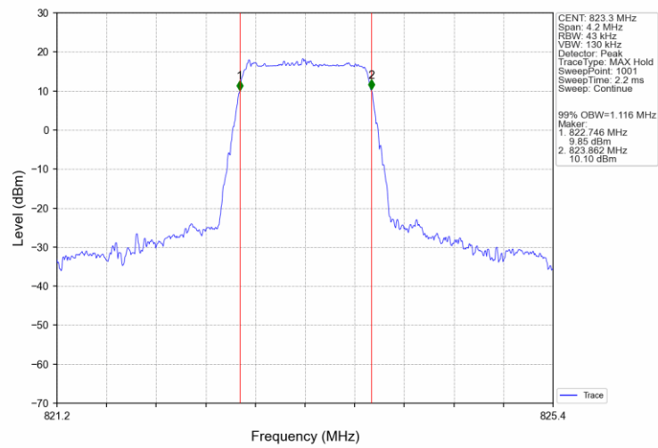
Band26a_1.4MHz_16QAM_HCH_823.3MHz_RB_6_0_NTNV
