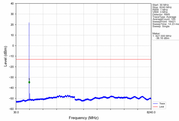
Band26a_1.4MHz_16QAM_HCH_823.3MHz_RB_1_0_NTNV
