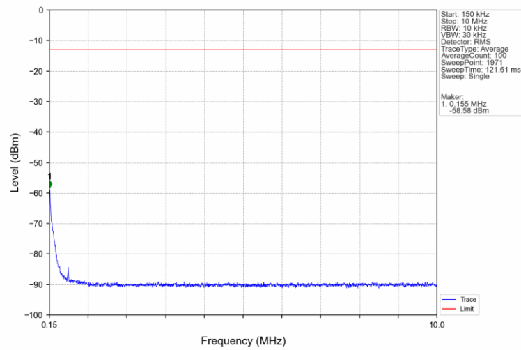
Band26a_1.4MHz_16QAM_MCH_819MHz_RB_1_0_NTNV
