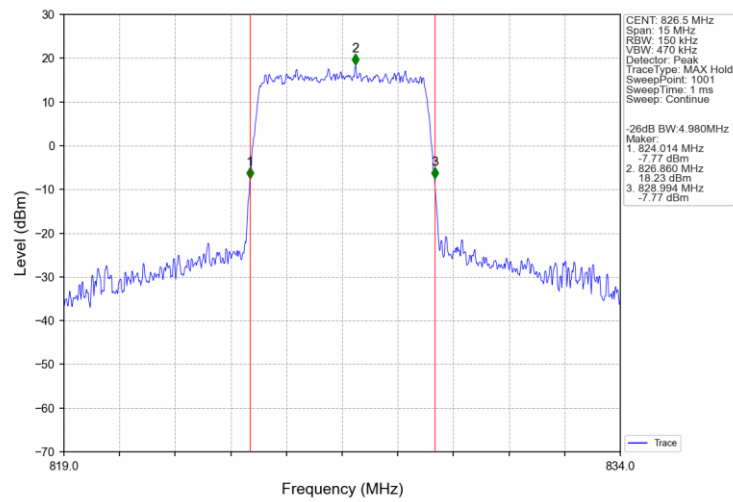
Band26b_5MHz_16QAM_LCH_826.5MHz_RB_25_0_NTNV
