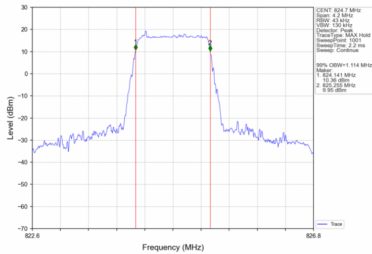
Band26b_1.4MHz_16QAM_LCH_824.7MHz_RB_6_0_NTNV
