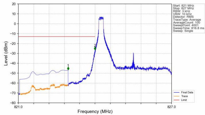
Band26b_3MHz_QPSK_LCH_825.5MHz_RB_1_0_NTNV
