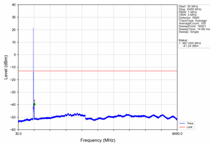
Band26b_15MHz_16QAM_MCH_836.5MHz_RB_1_0_NTNV
