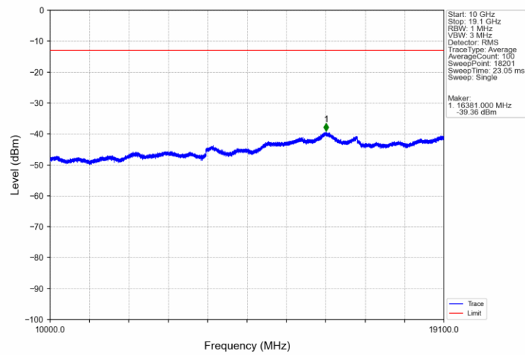
Band2_5MHz_16QAM_HCH_1907.5MHz_RB_1_0_NTNV
