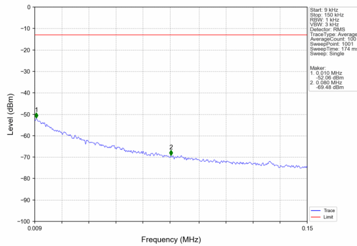
Band2_5MHz_16QAM_HCH_1907.5MHz_RB_1_0_NTNV
