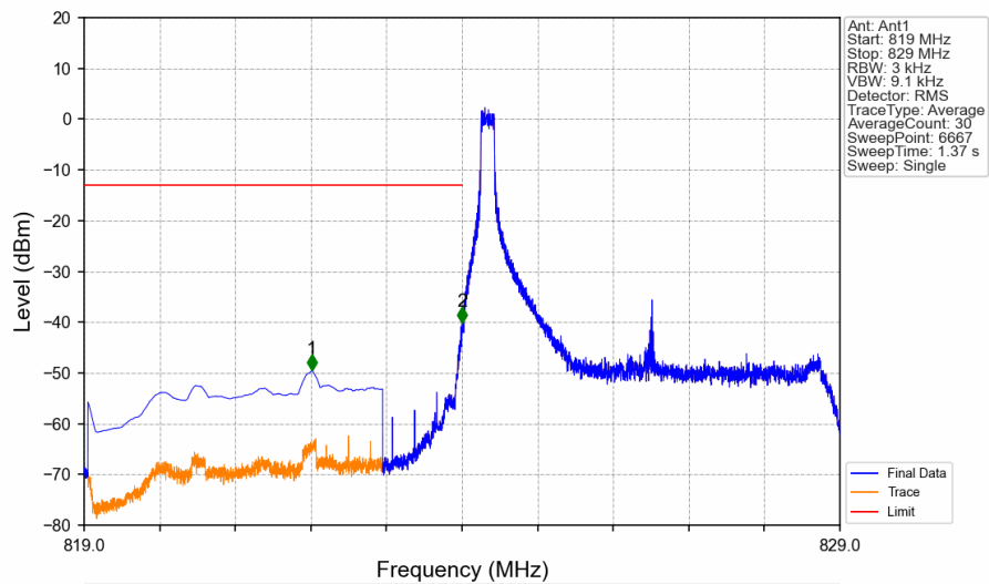
Band5_5MHz_QPSK_LCH_826.5MHz_RB_1_0_NTNV
