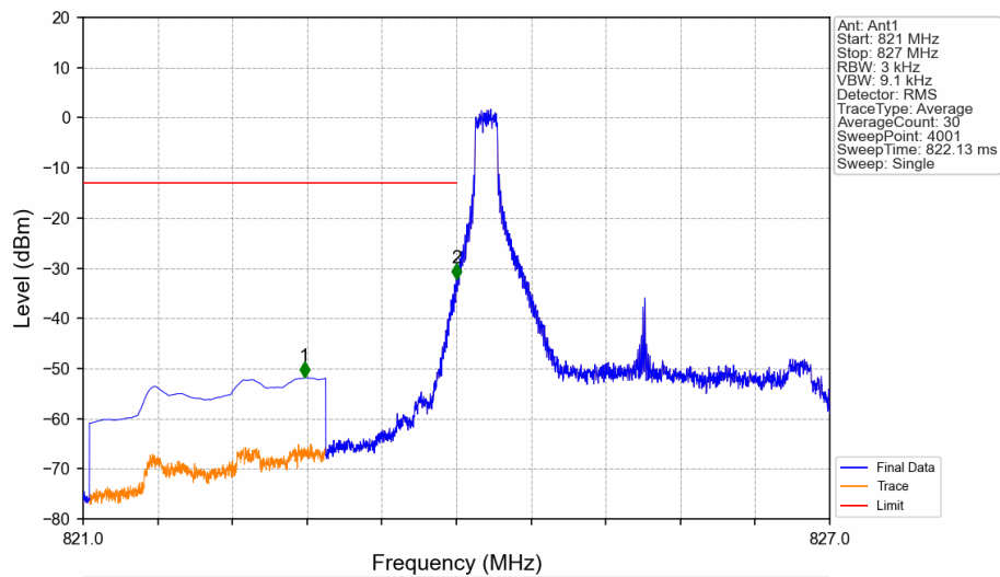
Band5_3MHz_QPSK_LCH_825.5MHz_RB_1_0_NTNV
