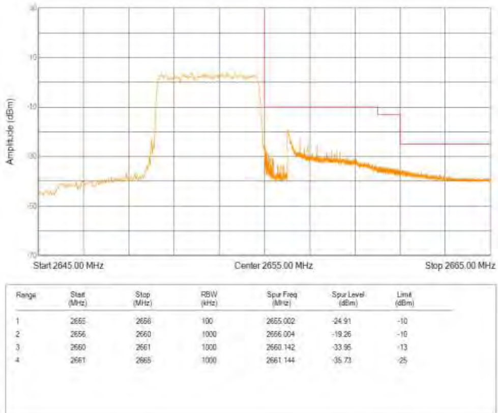
Band41(2655-2665) QPSK BW=5MHz Channel=40265 RB Size=25 Position=#0
