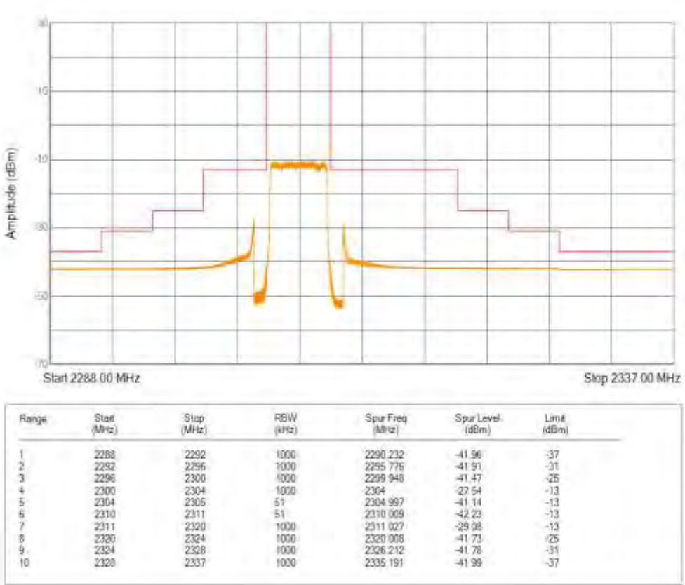
Band40(2305-2315) 16QAM BW=5MHz Channel=38775 RB Size=25 Position=#0
