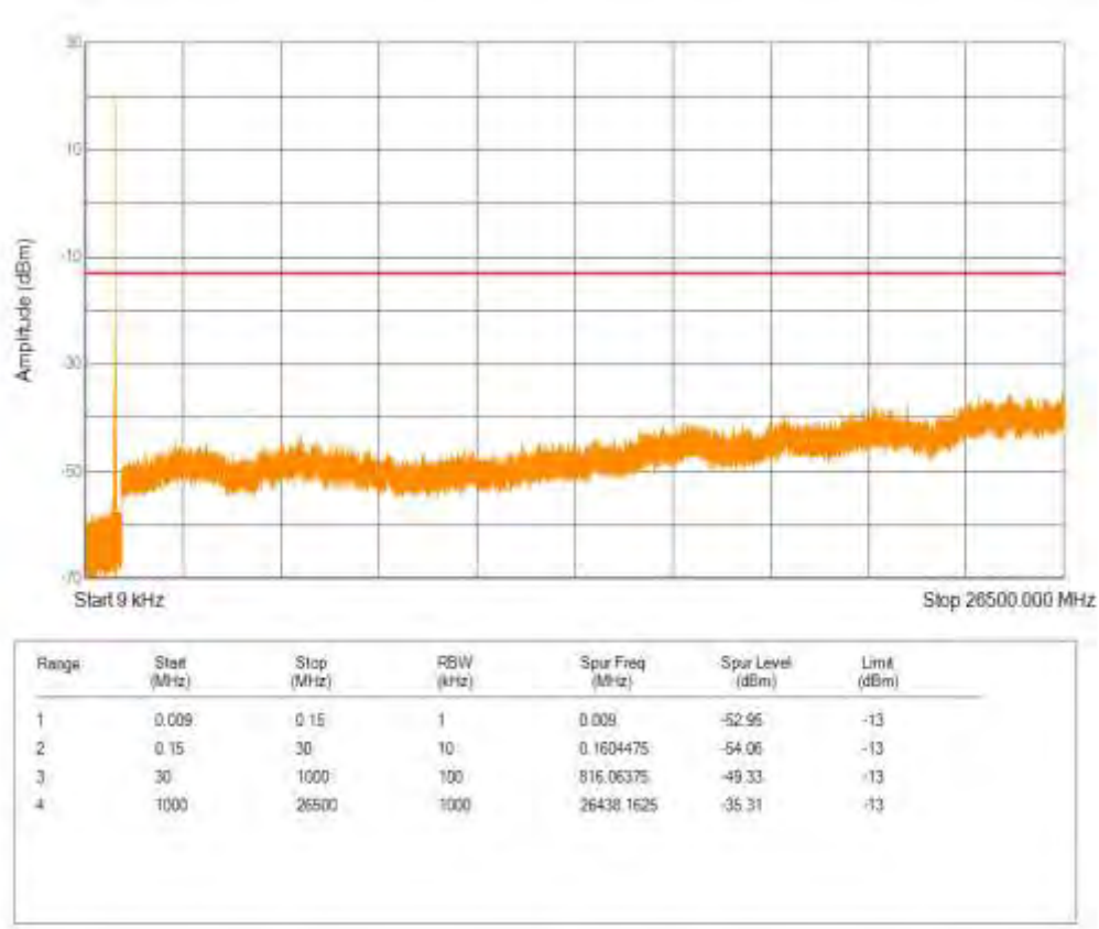
Band5 QAM16 BW=1.4MHz Channel=20643 RB Size=6 Position=#0
