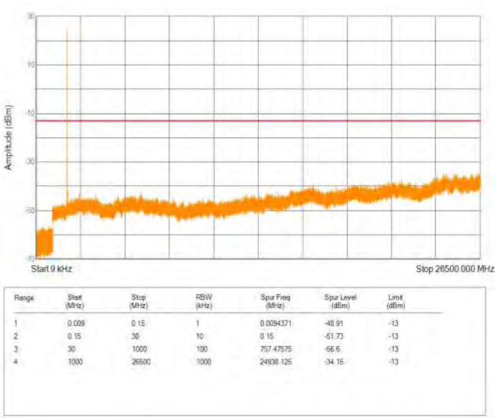
Band2 QPSK BW=5MHz Channel=18625 RB Size=25 Position=#0
