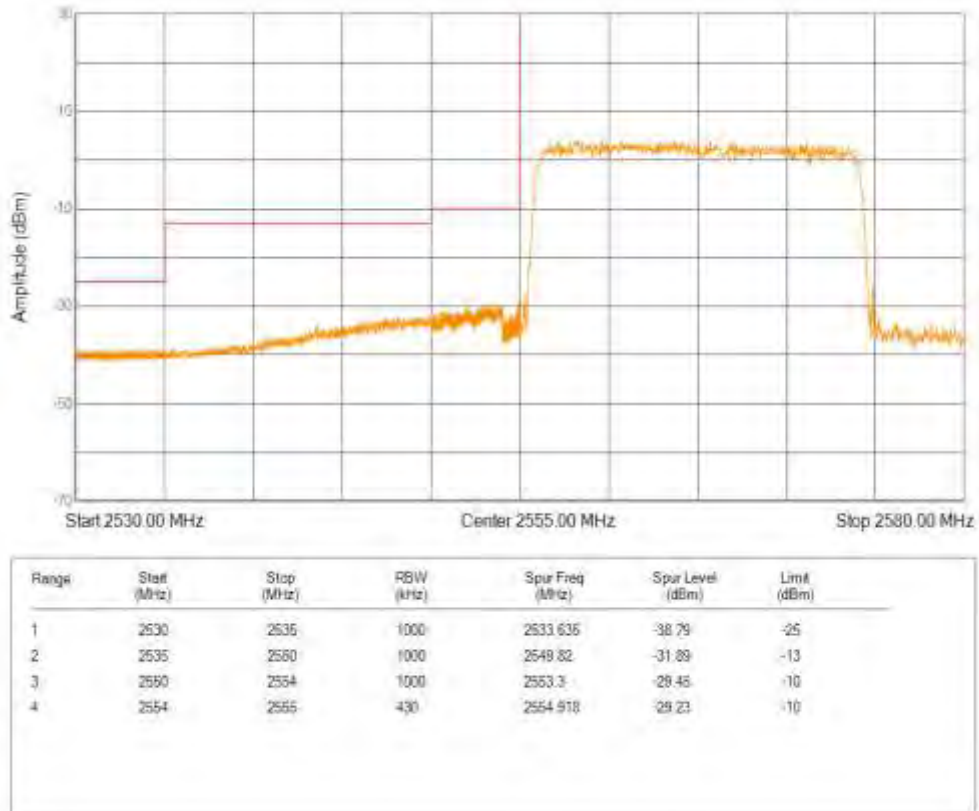
Band41(2555-2655) QAM16 BW=20MHz Channel=41140 RB Size=100 Position=#0
