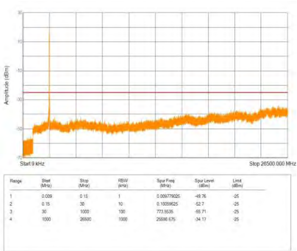
Band41(2555-2655) QAM16 BW=5MHz Channel=40265 RB Size=25 Position=#0
