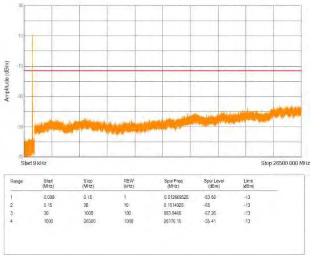
Band26(824-849) QAM16 BW=5MHz Channel=27015 RB Size=25 Position=#0
