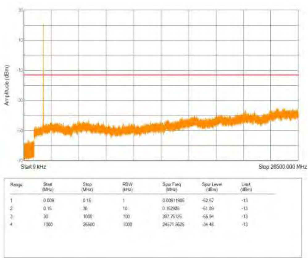
Band25 QPSK BW=15MHz Channel=26115 RB Size=75 Position=#0
