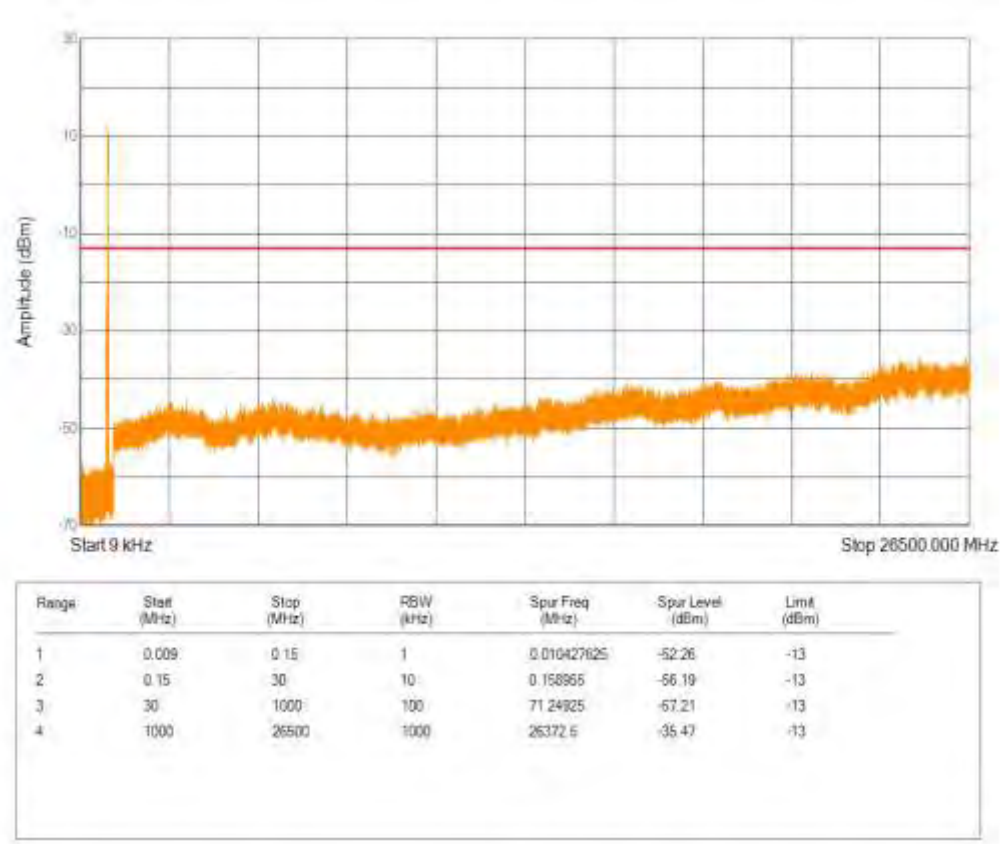
Band5 QAM16 BW=10MHz Channel=20600 RB Size=50 Position=#0
