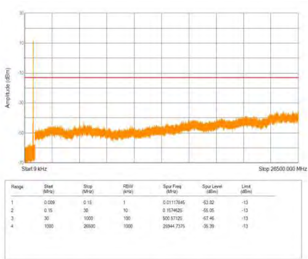
Band5 QAM16 BW=3MHz Channel=20415 RB Size=15 Position=#0
