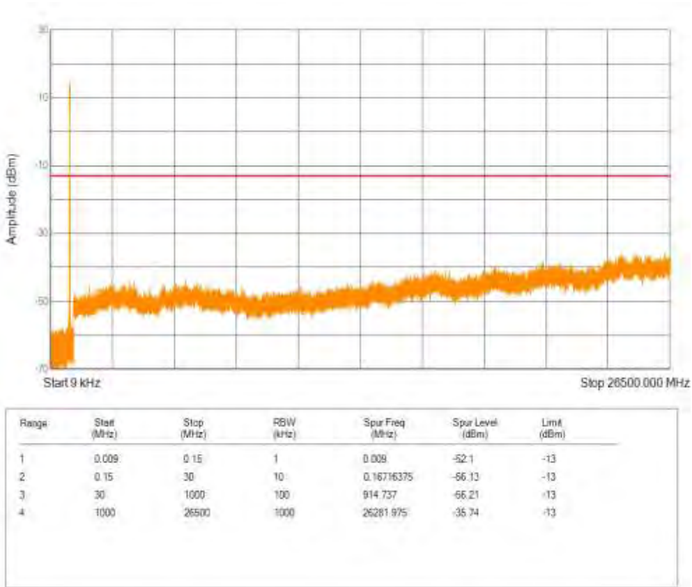
Band26(824-849) QAM16 BW=10MHz Channel=26990 RB Size=50 Position=#0
