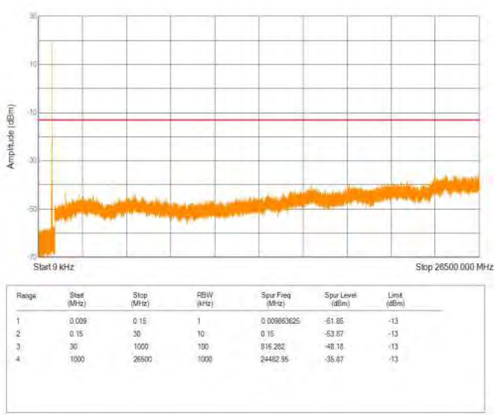
Band26(824-849) QAM16 BW=5MHz Channel=26815 RB Size=25 Position=#0
