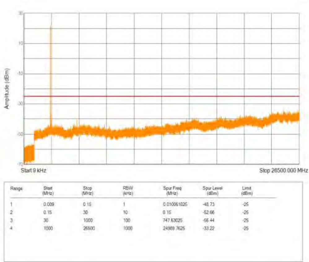
Band41(2555-2655) QAM16 BW=5MHz Channel=41215 RB Size=25 Position=#0
