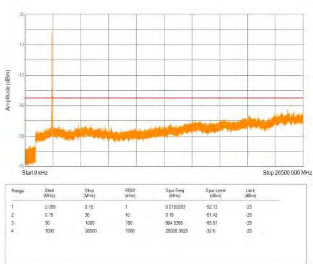
Band41(2555-2655) QPSK BW=15MHz Channel=41165 RB Size=75 Position=#0
