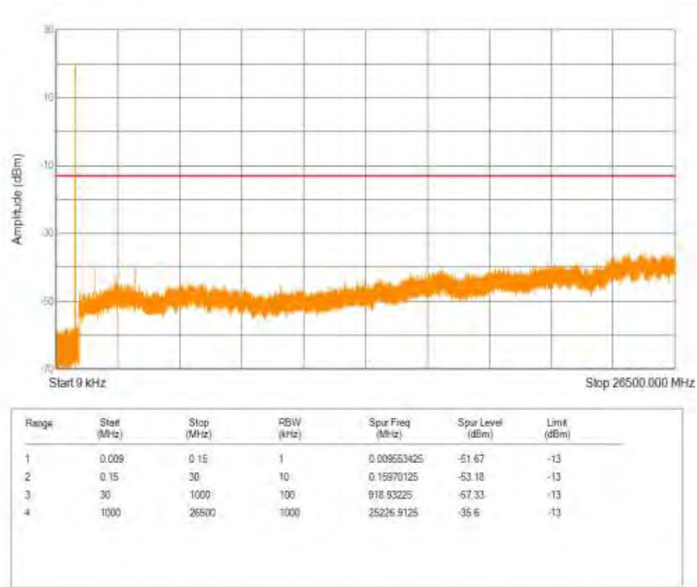
Band5 QAM16 BW=10MHz Channel=20450 RB Size=50 Position=#0
