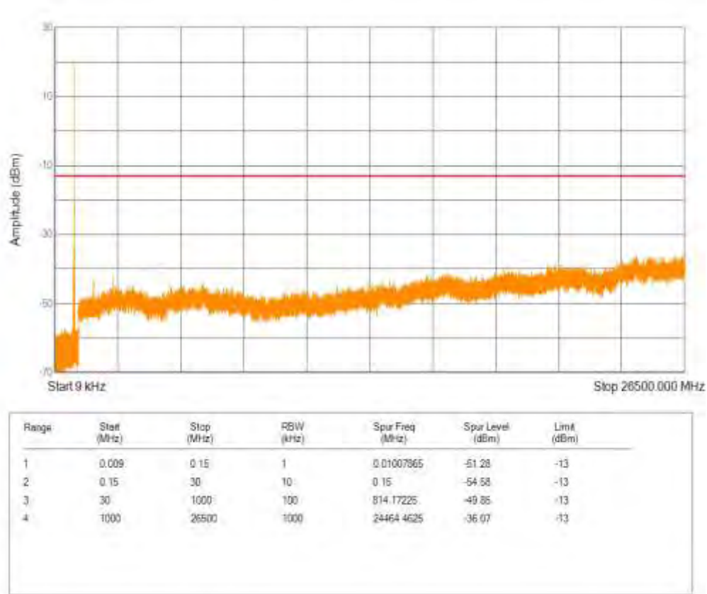
Band26(824-849) QPSK BW=1.4MHz Channel=27033 RB Size=6 Position=#0
