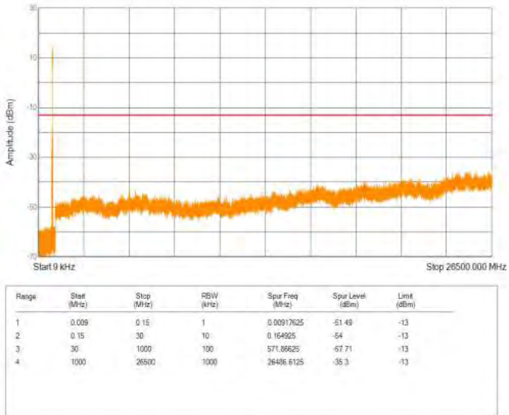
Band26(824-849) QAM16 BW=3MHz Channel=27025 RB Size=15 Position=#0
