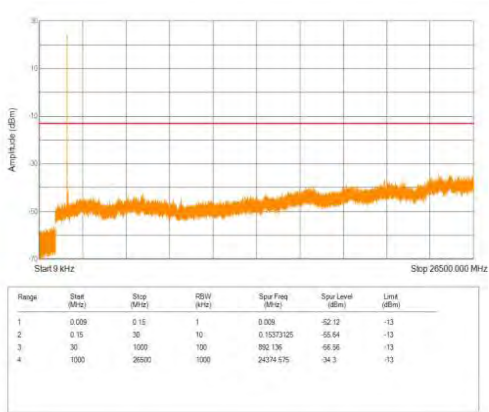
Band4 QAM16 BW=5MHz Channel=19975 RB Size=25 Position=#0
