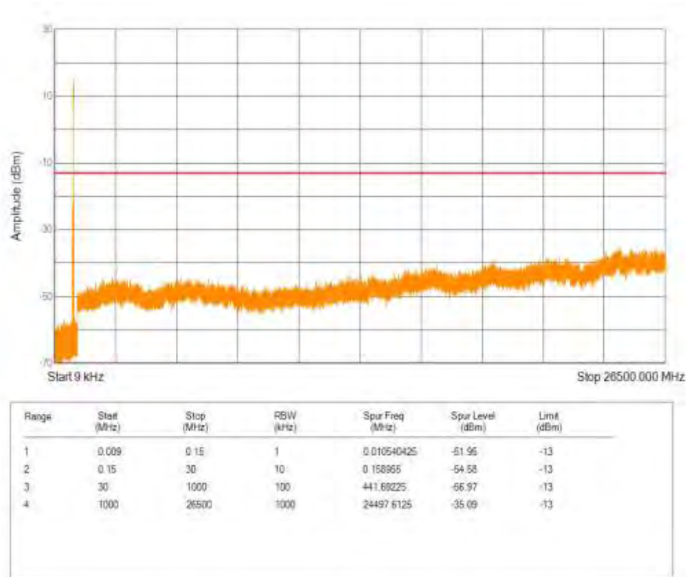
Band5 QPSK BW=5MHz Channel=20625 RB Size=25 Position=#0
