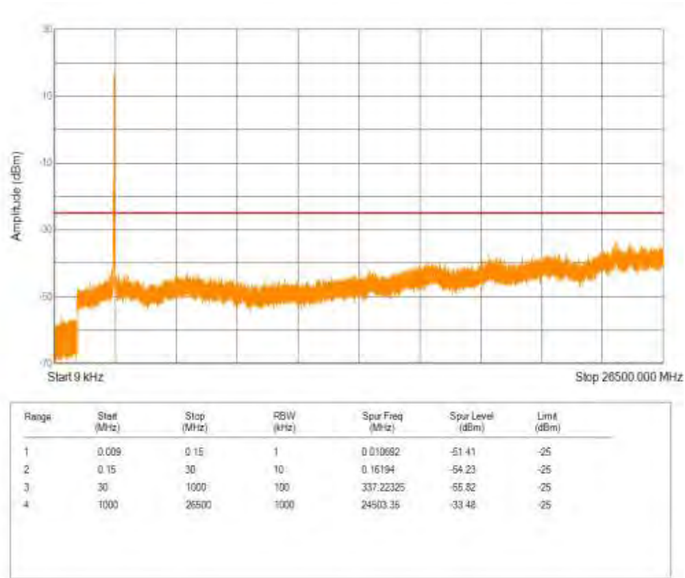
Band38 QAM16 BW=5MHz Channel=37775 RB Size=25 Position=#0
