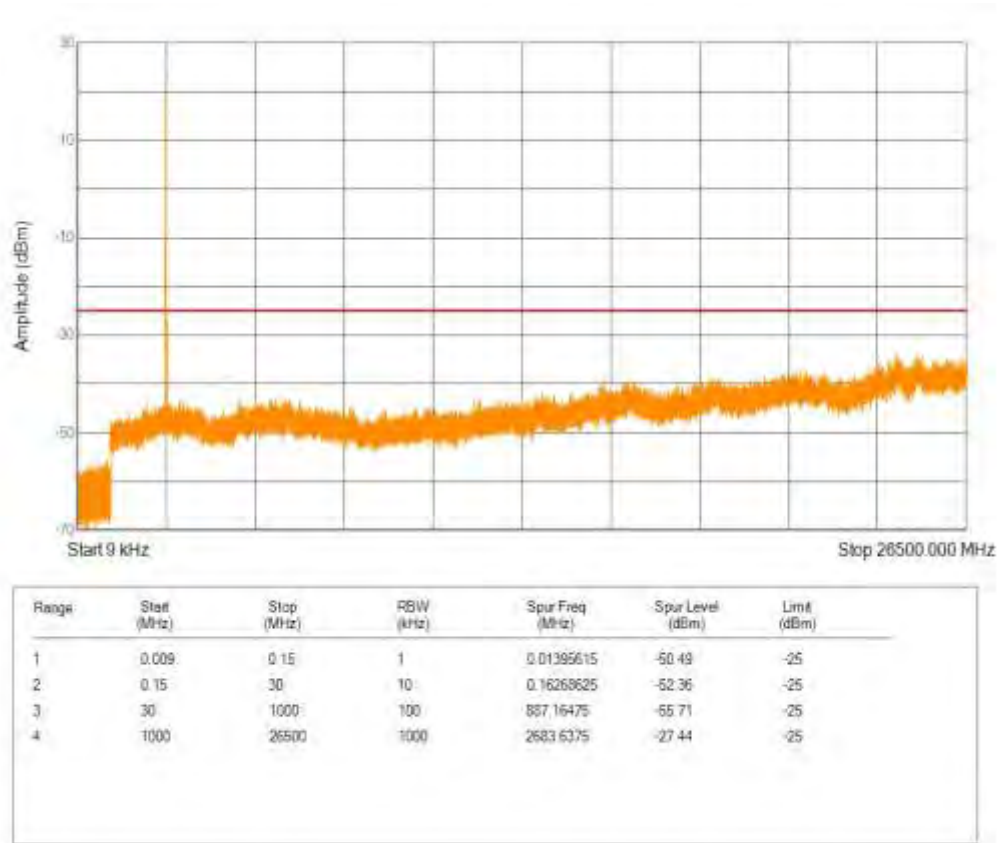
Band5 QAM16 BW=1.4MHz Channel=20407 RB Size=6 Position=#0
