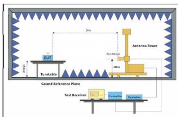
Above 1GHz
