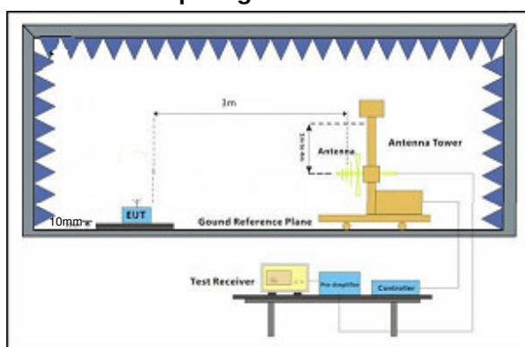
Below 1GHz
