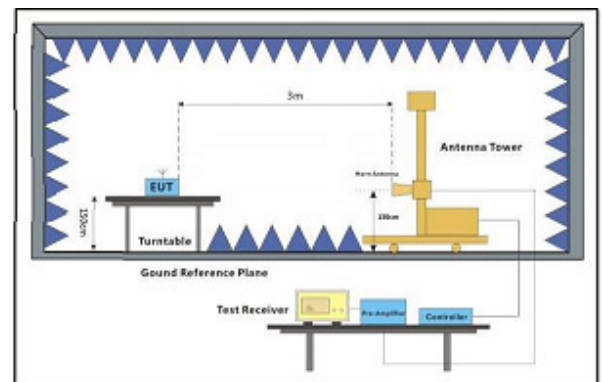
Above 1GHz
