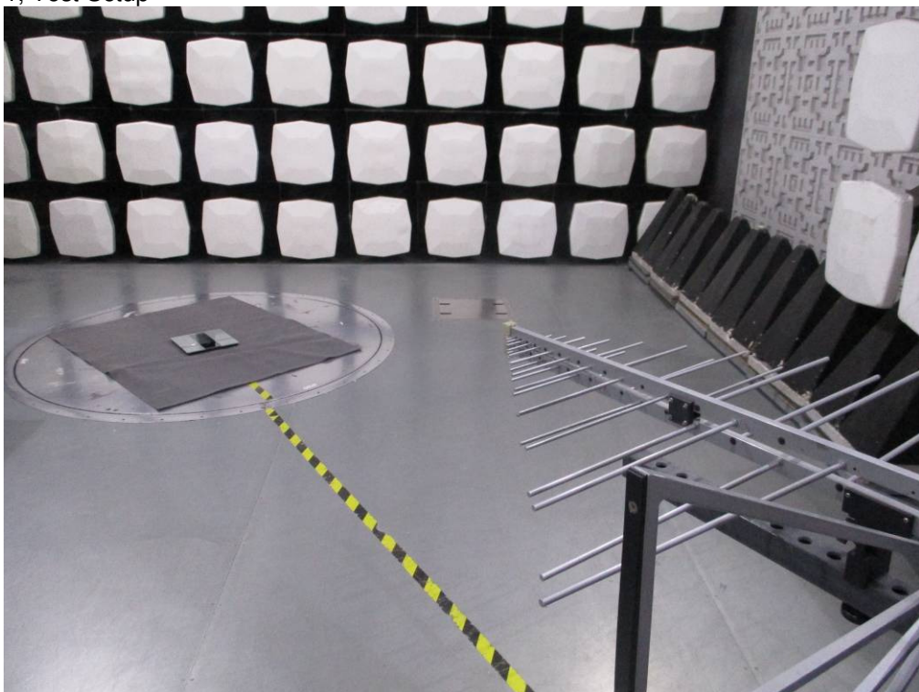
1, Test Setup
