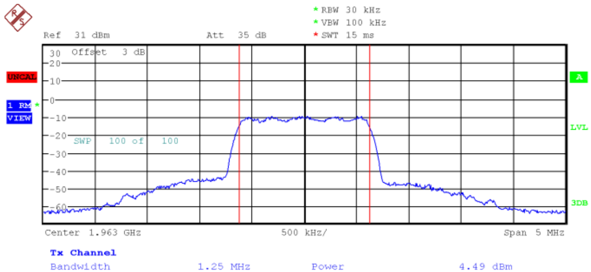
Plot C Downlink / 1963.00MHz / CDMA
