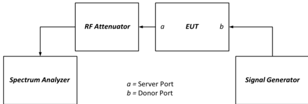
Figure 5 – Test setup for downlink noise power measurement in the presence of a downlink signal
