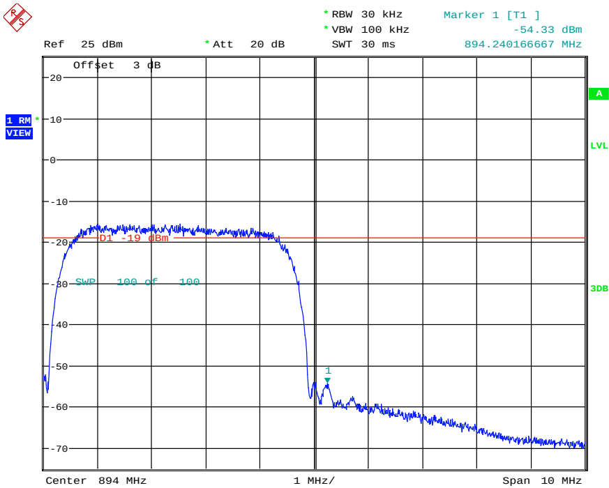
Plot A5 Downlink / GSM / 893.8MHz
