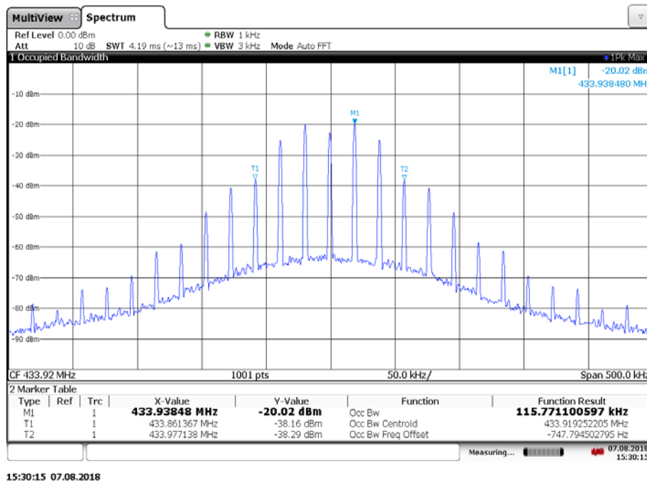
Plot 3: 99 % emission bandwidth, Channel 1
