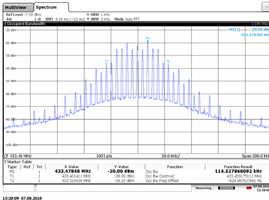
Plot 1: 99 % emission bandwidth, Channel 0
