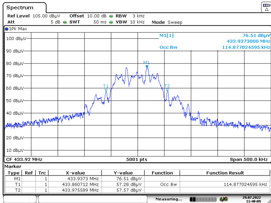
Plot 1: Emissions bandwidth – low channel
