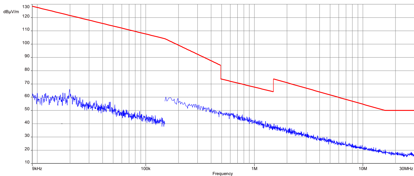
Plot 4: 9 kHz to 30 MHz high channel
