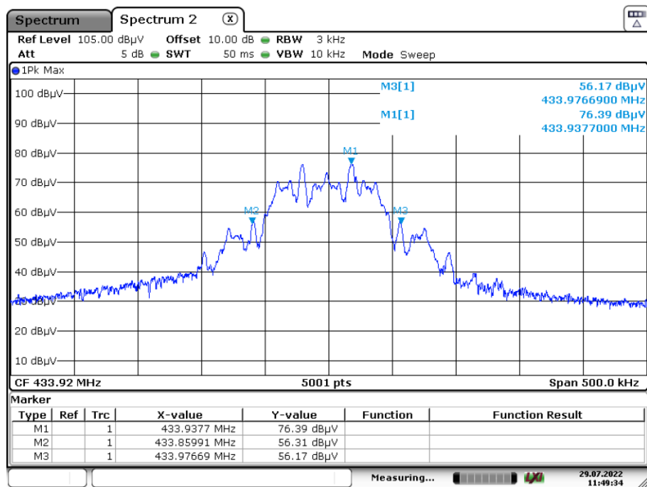
Plot 2: 99 % emission bandwidth – low channel
