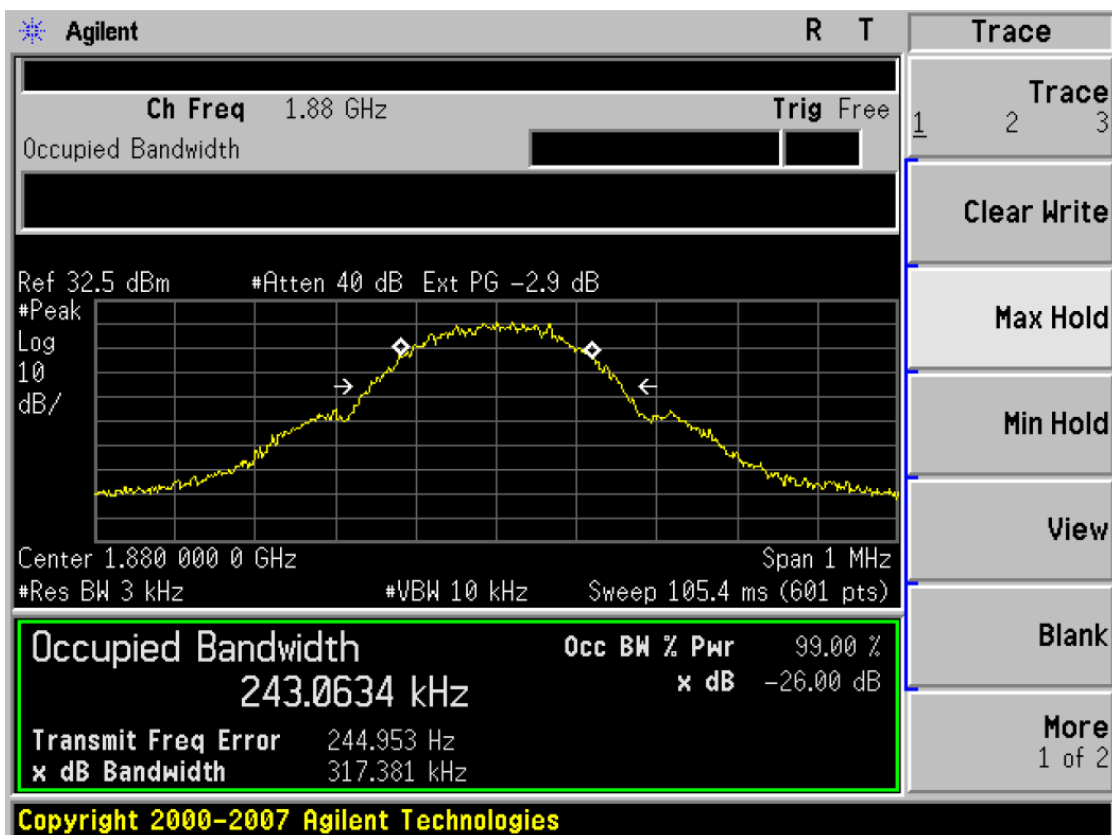
(Plot 4.3.4 B: Channel 661:1880.00MHz @ GPRS1900)
