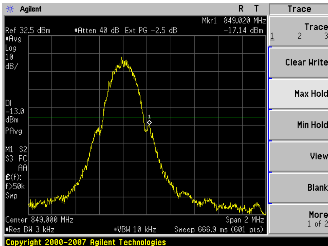
(Plot 4.4.1 B: Channel 251: 848.80MHz @ GSM850)
