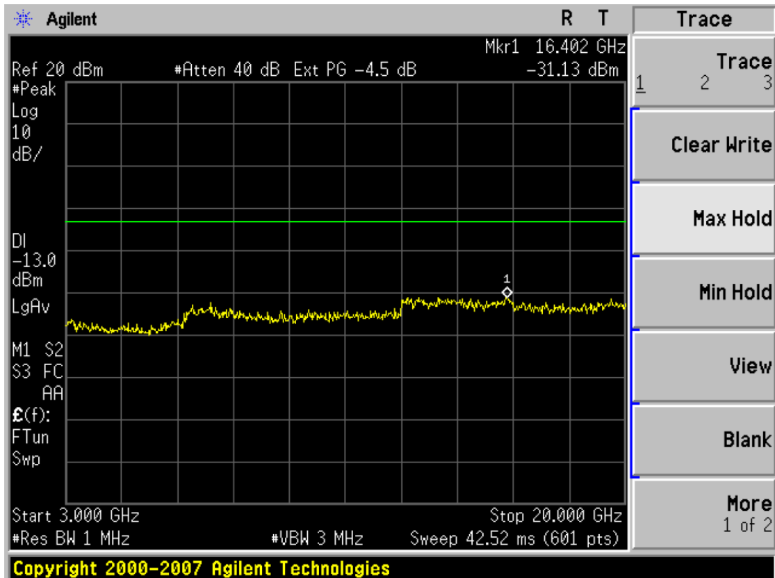
(Plot 4.5.2 B2: Channel 661: 1880.00MHz @ Traffic @ PCS1900)
