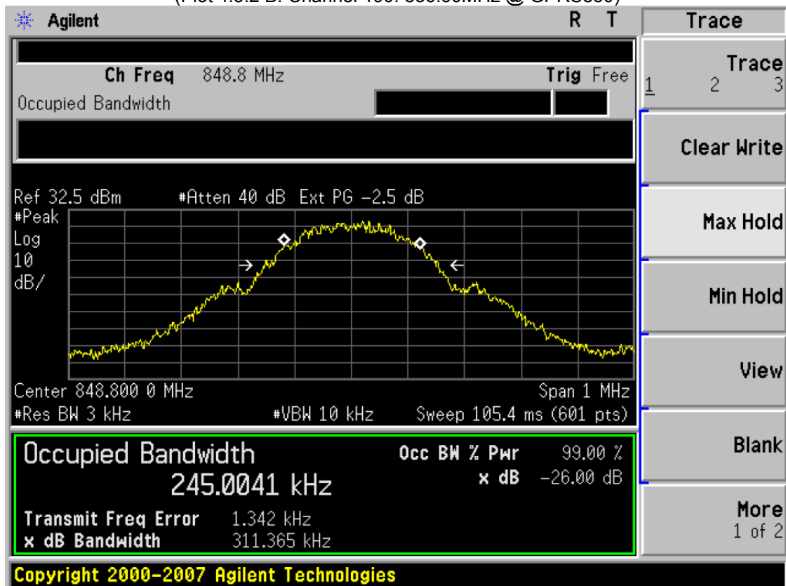
(Plot 4.3.2 C: Channel 251: 848.80MHz @ GPRS850)
