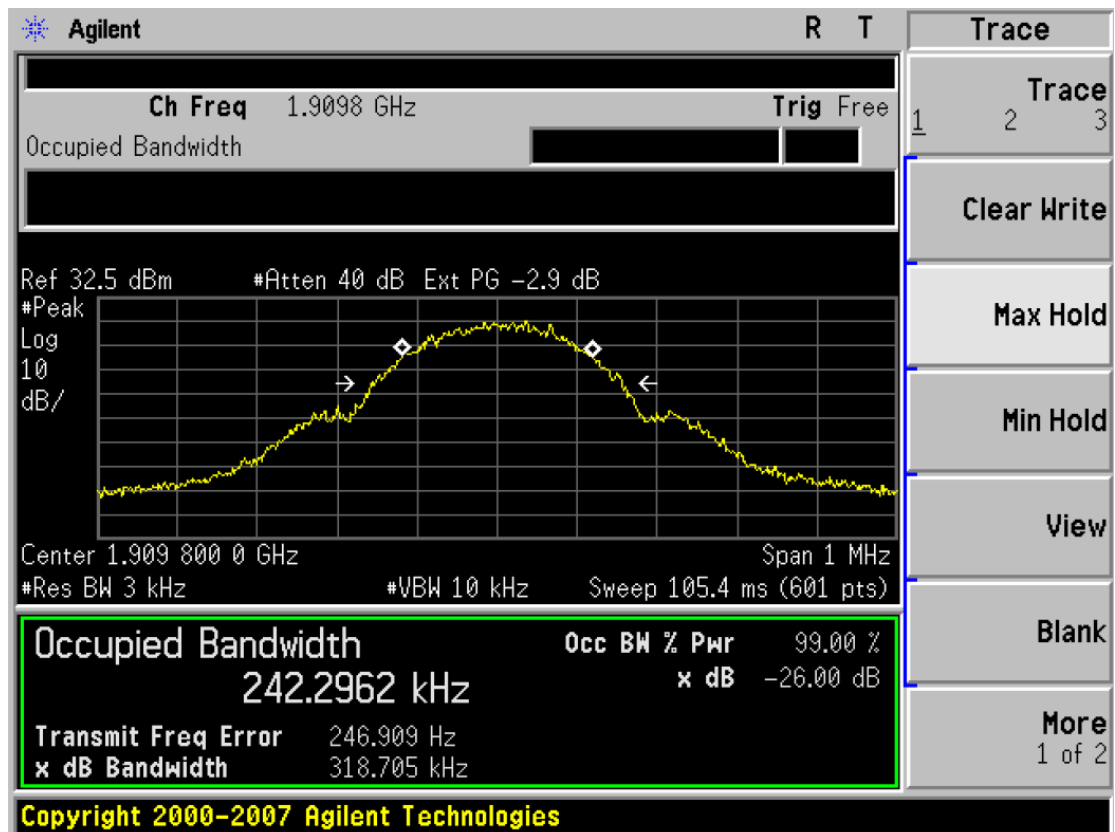
(Plot 4.3.4 C: Channel 810:1909.80MHz @ GPRS1900)
