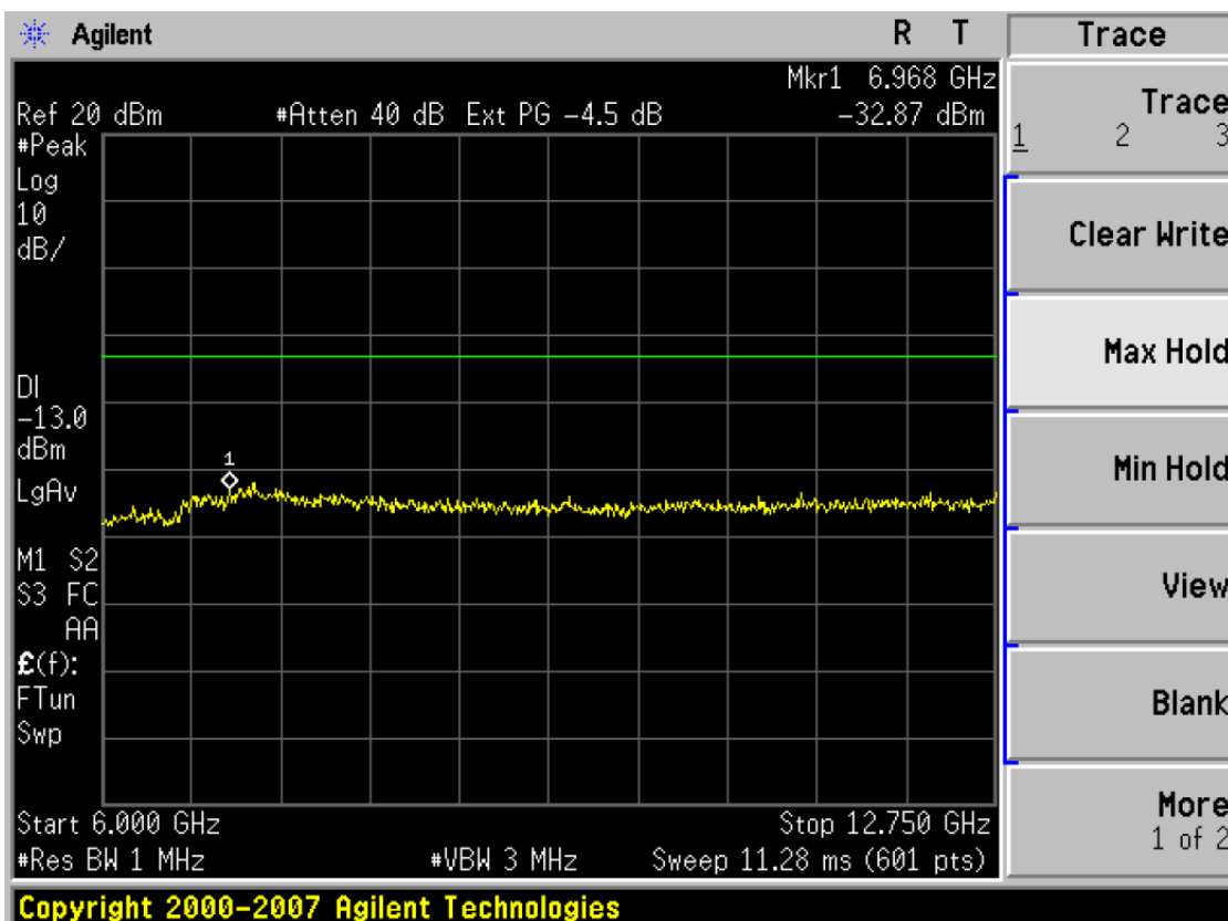
(Plot 4.5.1 A3: Channel 128: 824.20MHz @ Traffic @ GSM850)
