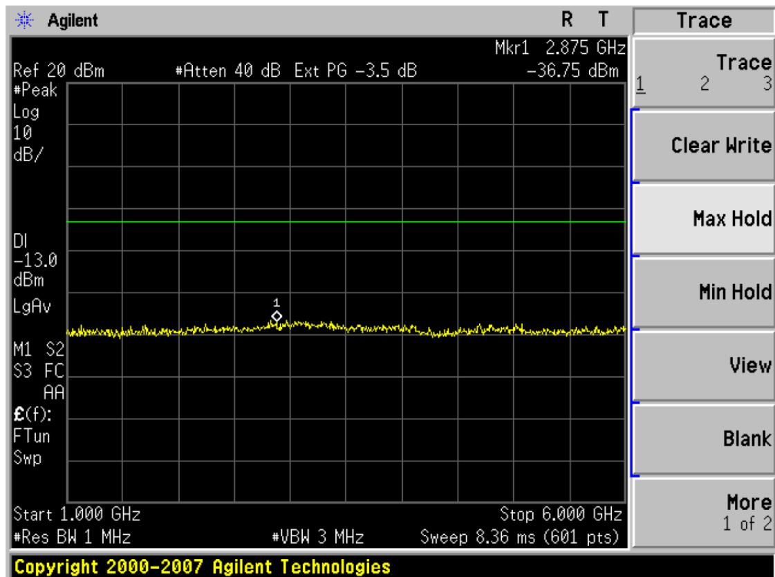
(Plot 4.5.1 C2: Channel 251: 848.80MHz @ Traffic @ GSM850)
