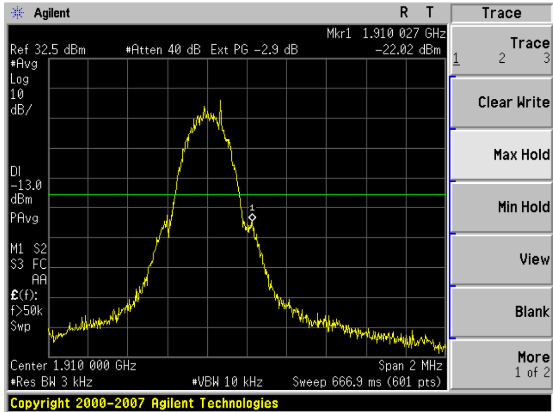
(Plot 4.4.4 B: Channel 810: 1909.80MHz @ GPRS1900)
