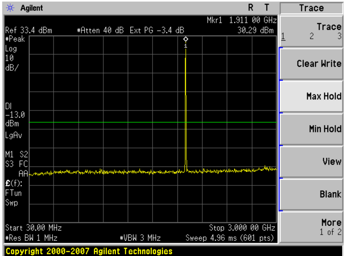
(Plot 4.5.2 C1: Channel 810: 1909.80MHz @ Traffic @ PCS1900)
