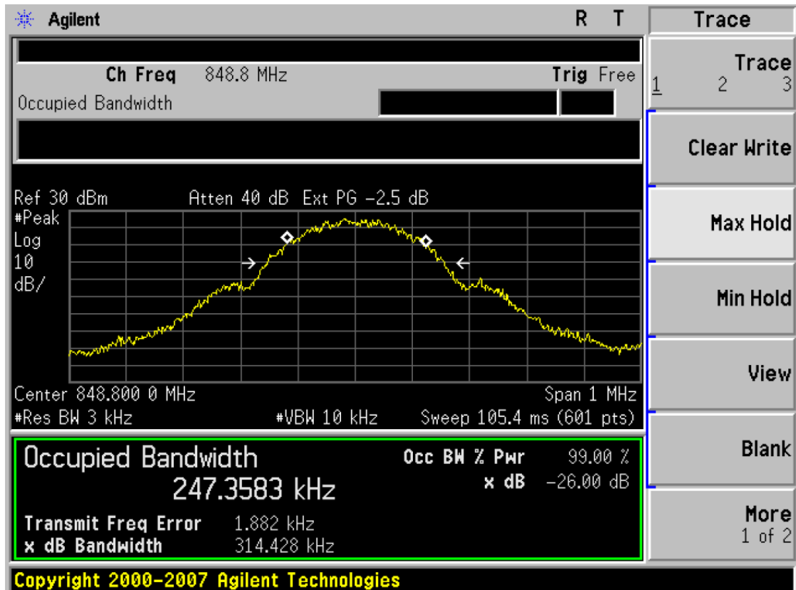
(Plot 4.3.1 C: Channel 251: 848.80MHz @ GSM850)
