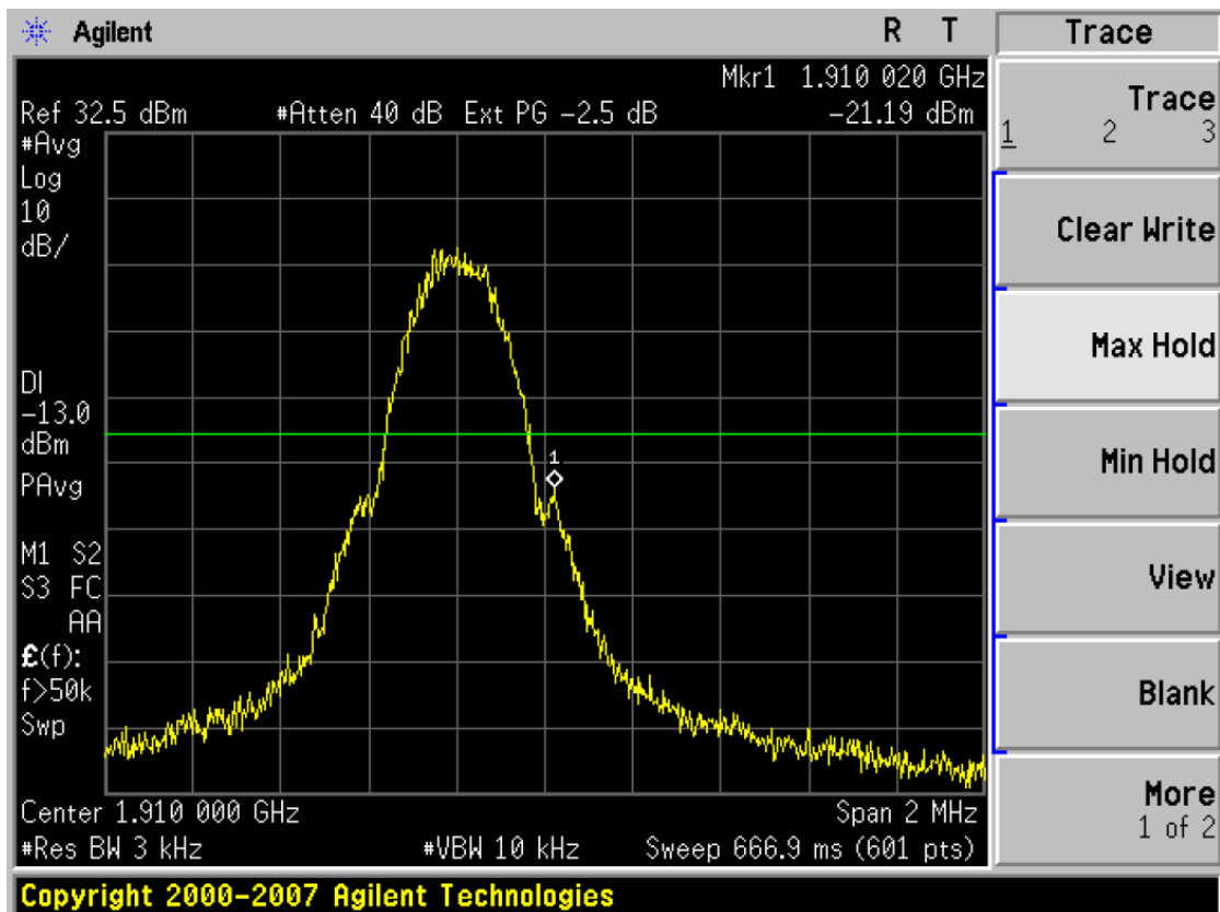
(Plot 4.4.3 B: Channel 810: 1909.80MHz @ PCS1900)
