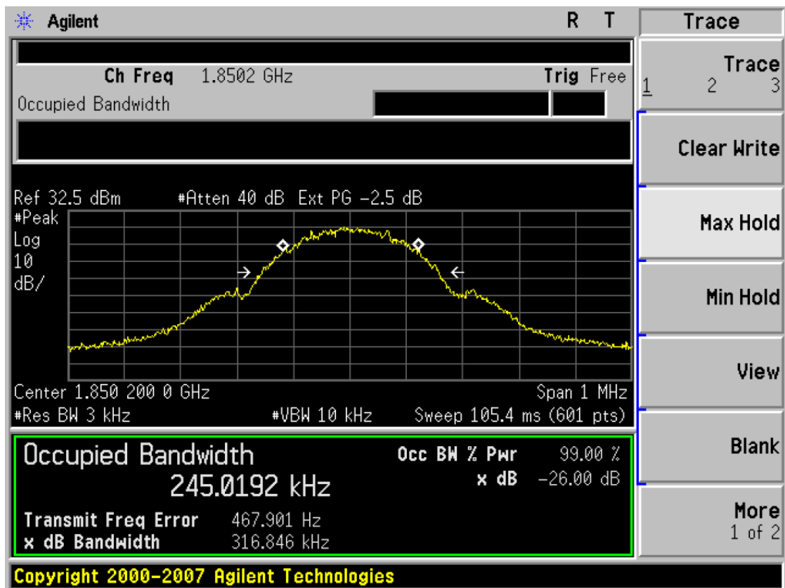
(Plot 4.3.3 A: Channel 512:1820.20MHz @ PCS1900)
