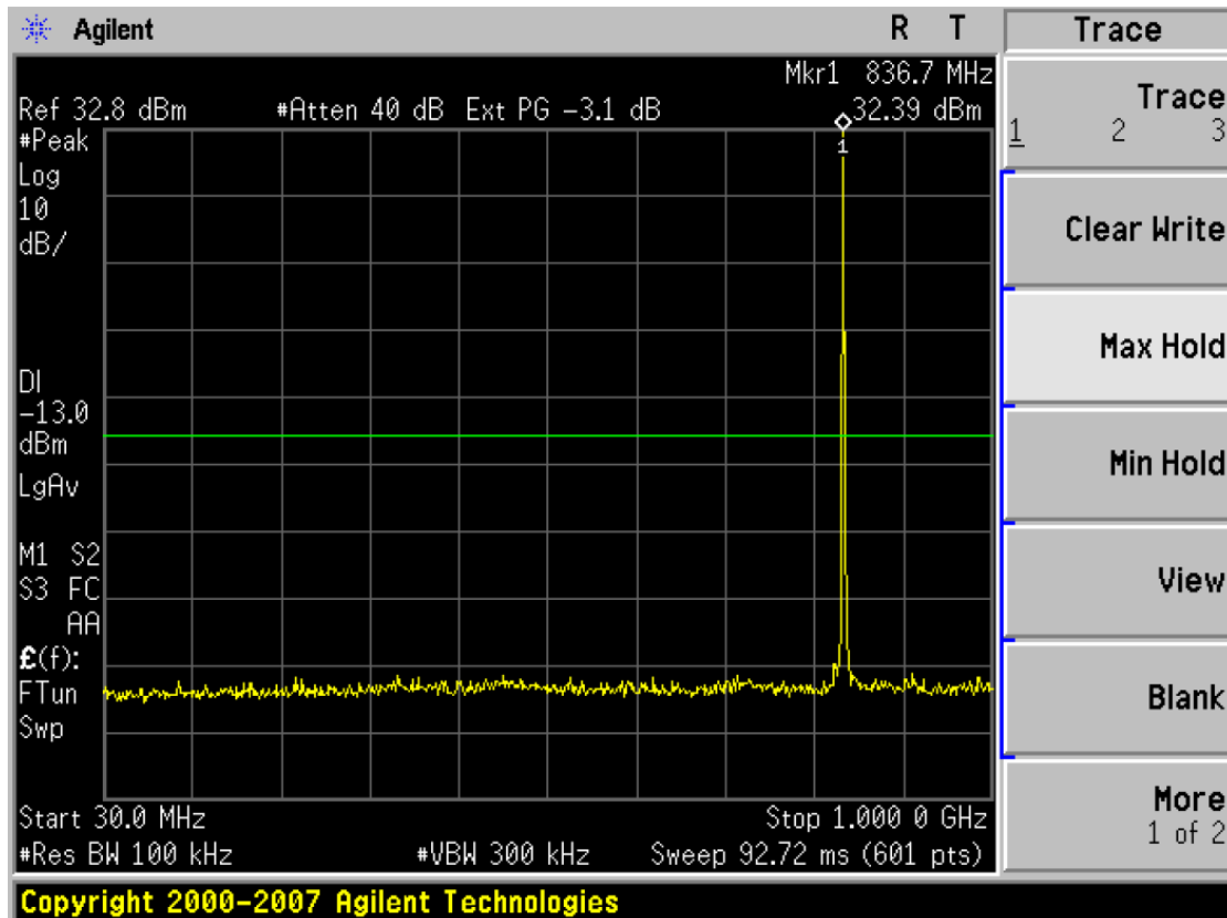
(Plot 4.5.1 B1: Channel 190: 836.60MHz @ Traffic @ GSM850)
