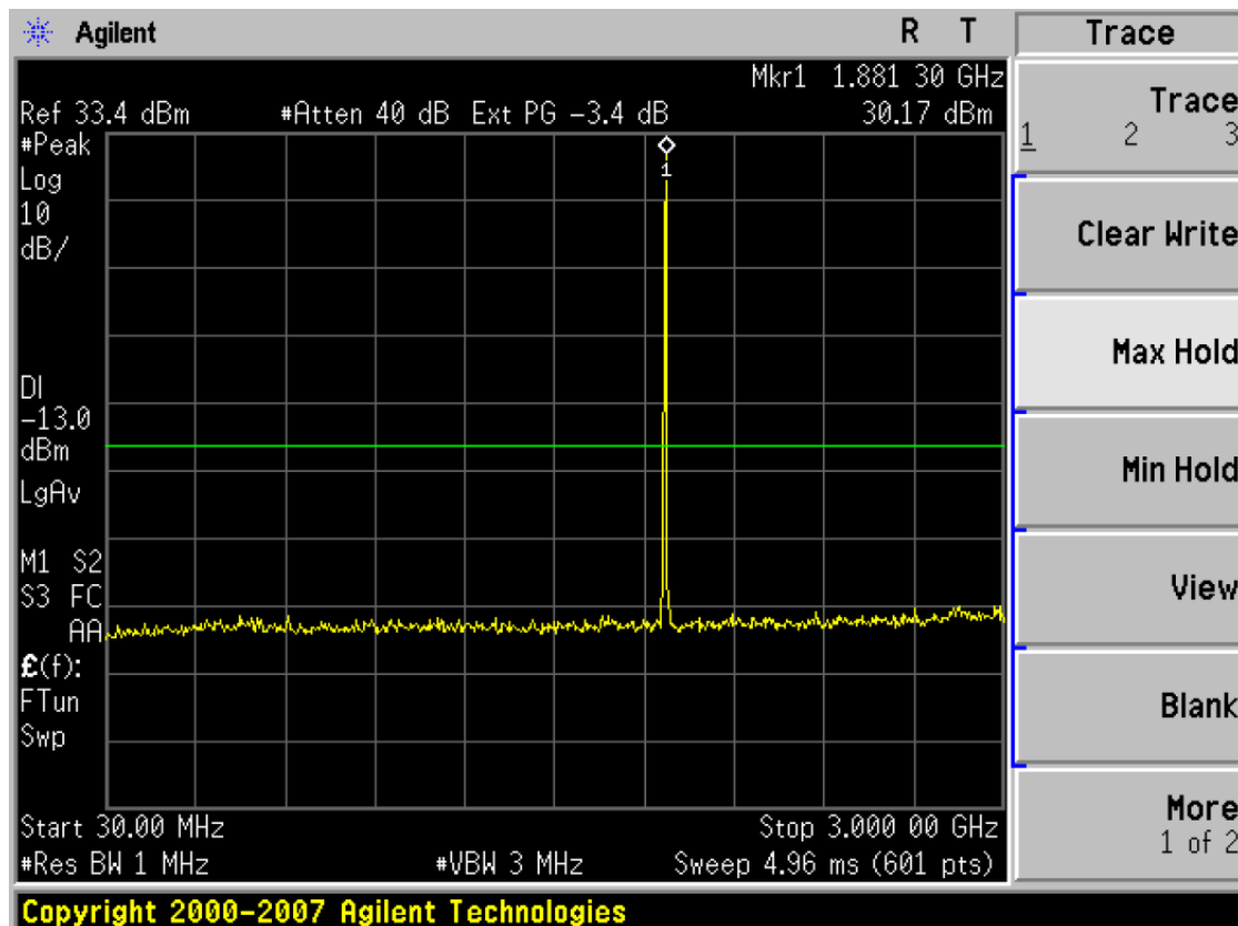
(Plot 4.5.2 B1: Channel 661: 1880.00MHz @ Traffic @ PCS1900)
