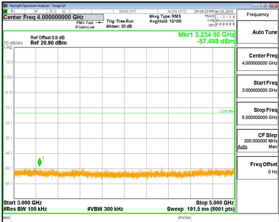
(Plot 4.5.1 A3: Channel 00: 2402MHz @ GFSK)
