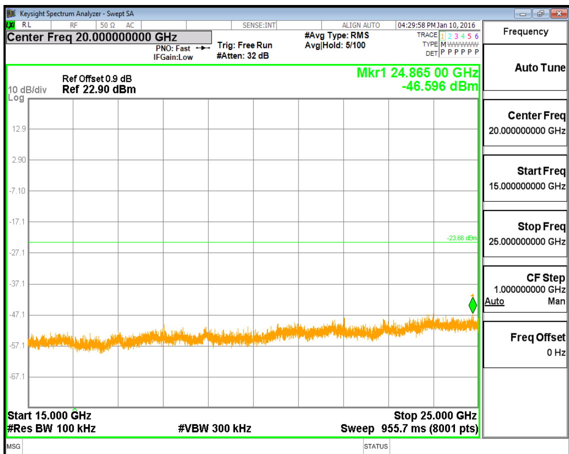
(Plot 4.5.1 C6: Channel 39: 2480MHz @ GFSK)
