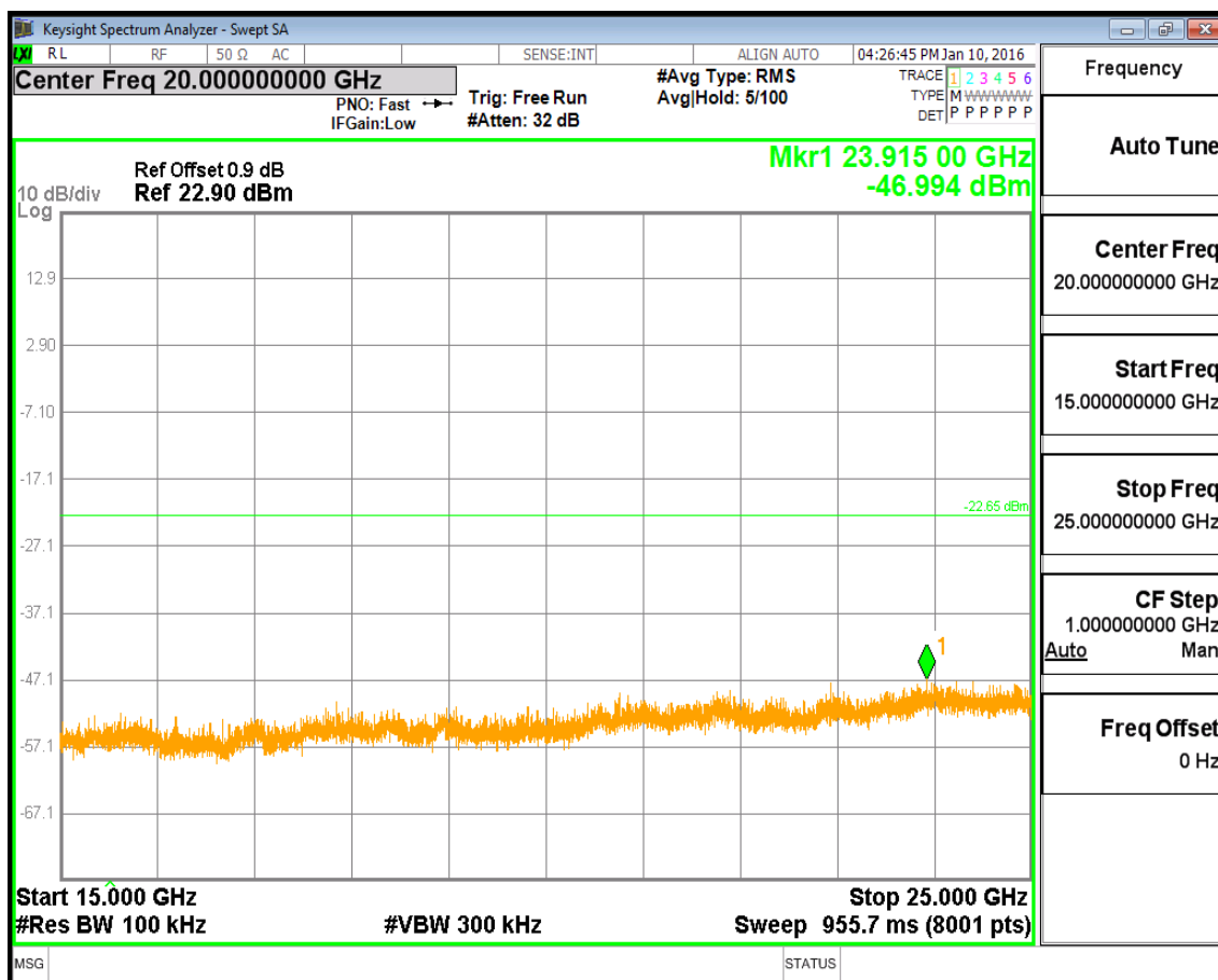
(Plot 4.5.1 A6: Channel 00: 2402MHz @ GFSK)
