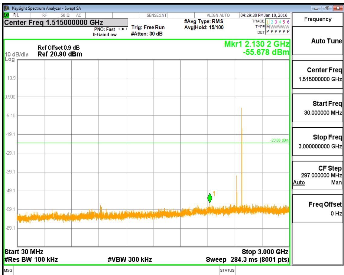
(Plot 4.5.1 C2: Channel 39: 2480MHz @ GFSK)
