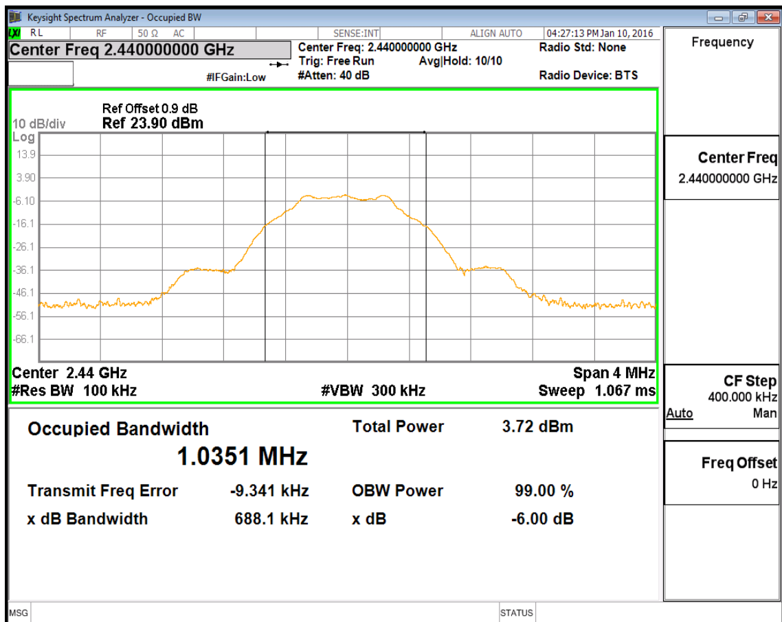
(Plot 4.6.1 B: Channel 19: 2440MHz @ GFSK)
