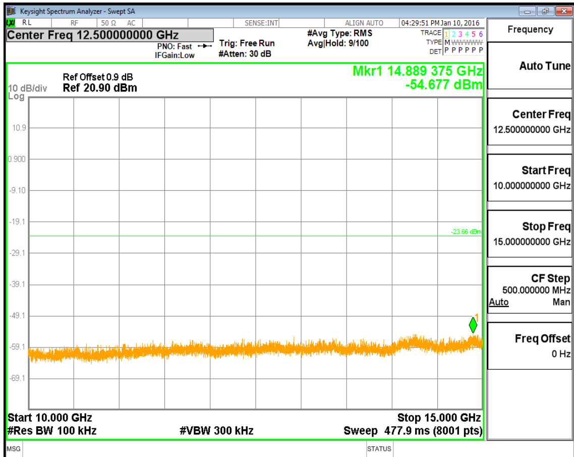
(Plot 4.5.1 C5: Channel 39: 2480MHz @ GFSK)
