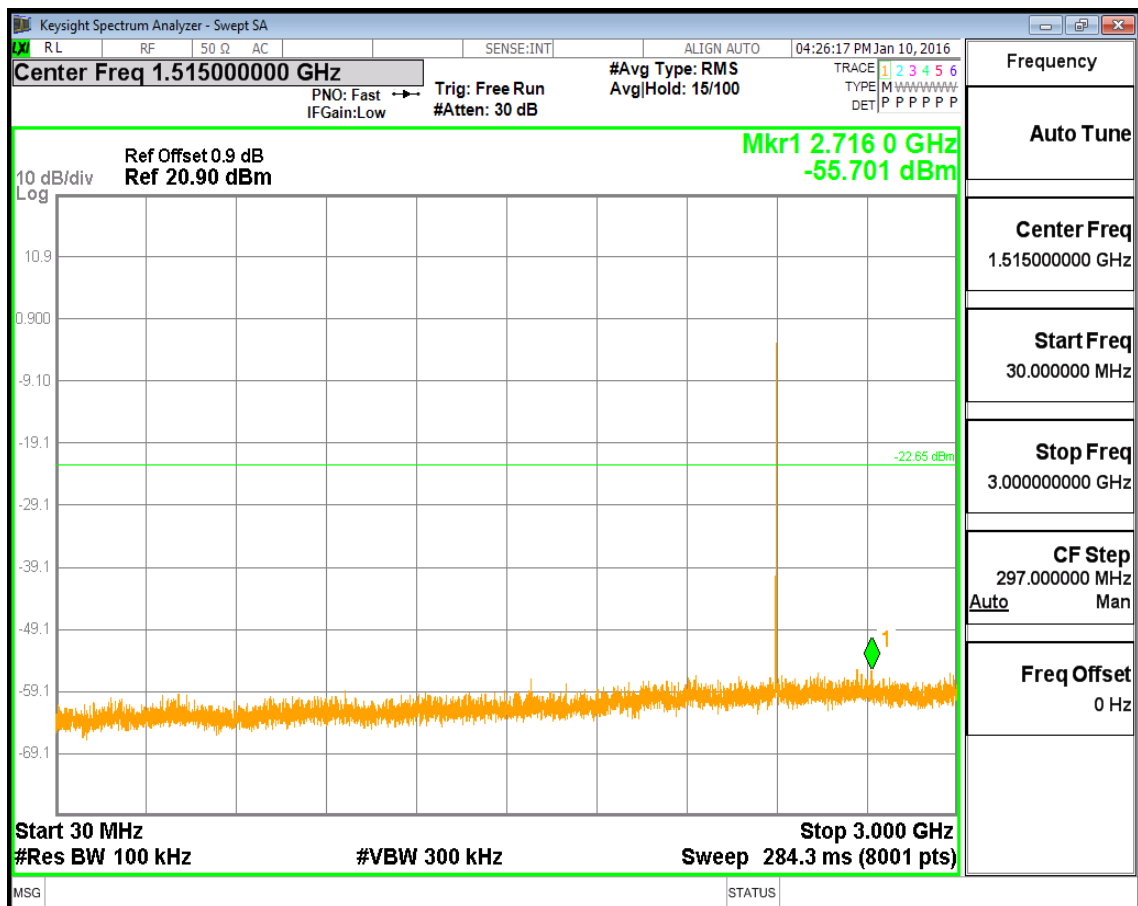
(Plot 4.5.1 A2: Channel 00: 2402MHz @ GFSK)
