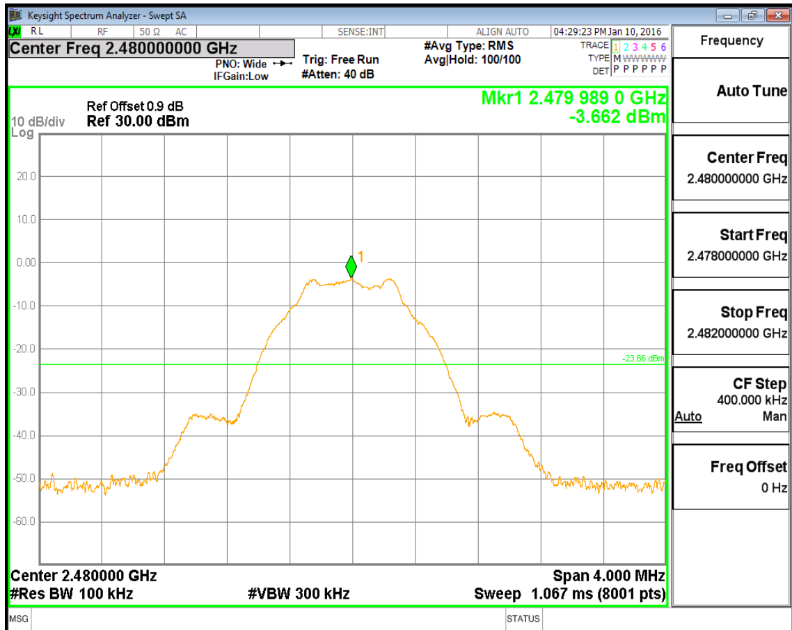
(Plot 4.5.1 C1: Channel 39: 2480MHz @ GFSK)
