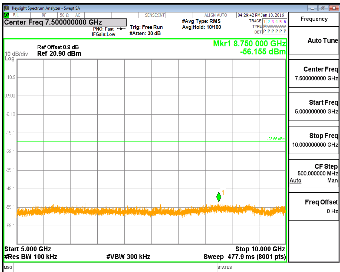
(Plot 4.5.1 C4: Channel 39: 2480MHz @ GFSK)
