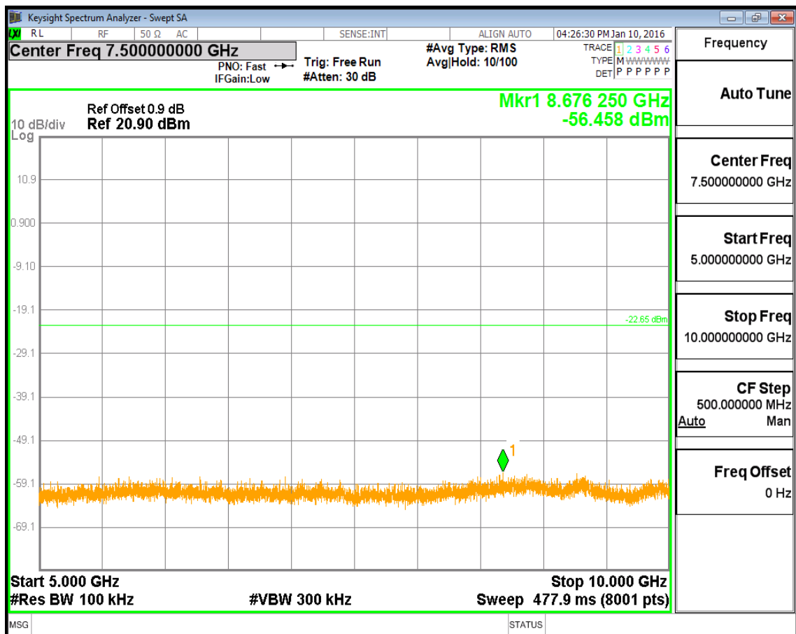
(Plot 4.5.1 A4: Channel 00: 2402MHz @ GFSK)
