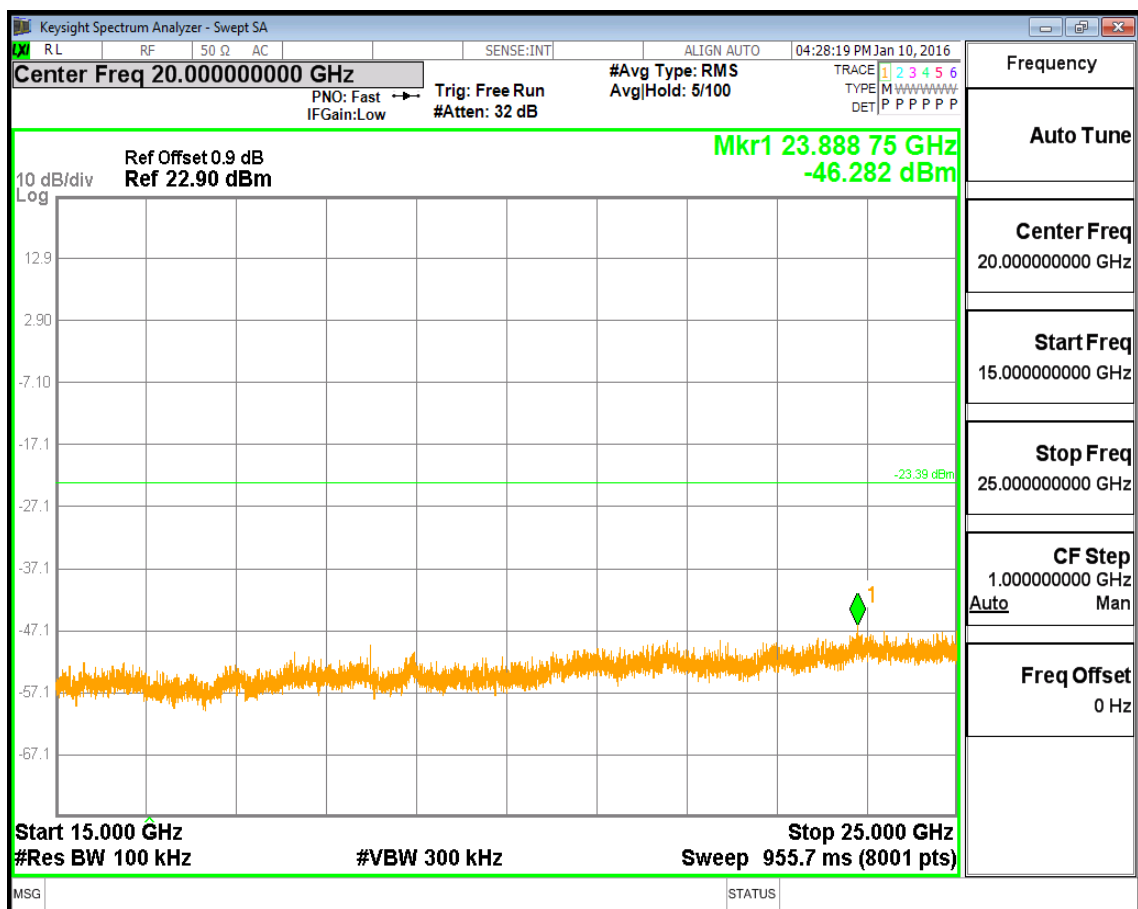
(Plot 4.5.1 B6: Channel 19: 2440MHz @ GFSK)
