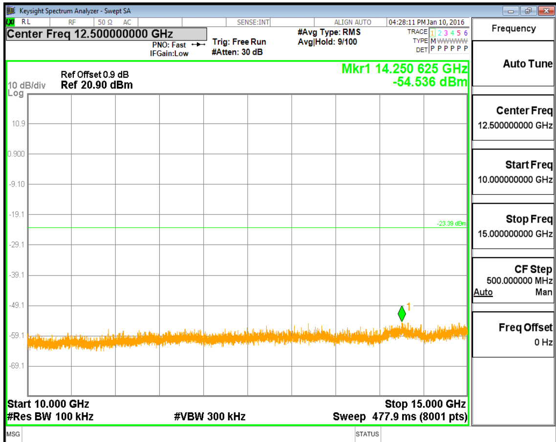
(Plot 4.5.1 B5: Channel 19: 2440MHz @ GFSK)
