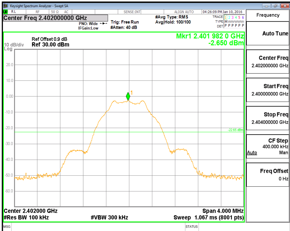
(Plot 4.5.1 A1: Channel 00: 2402MHz @ GFSK)
