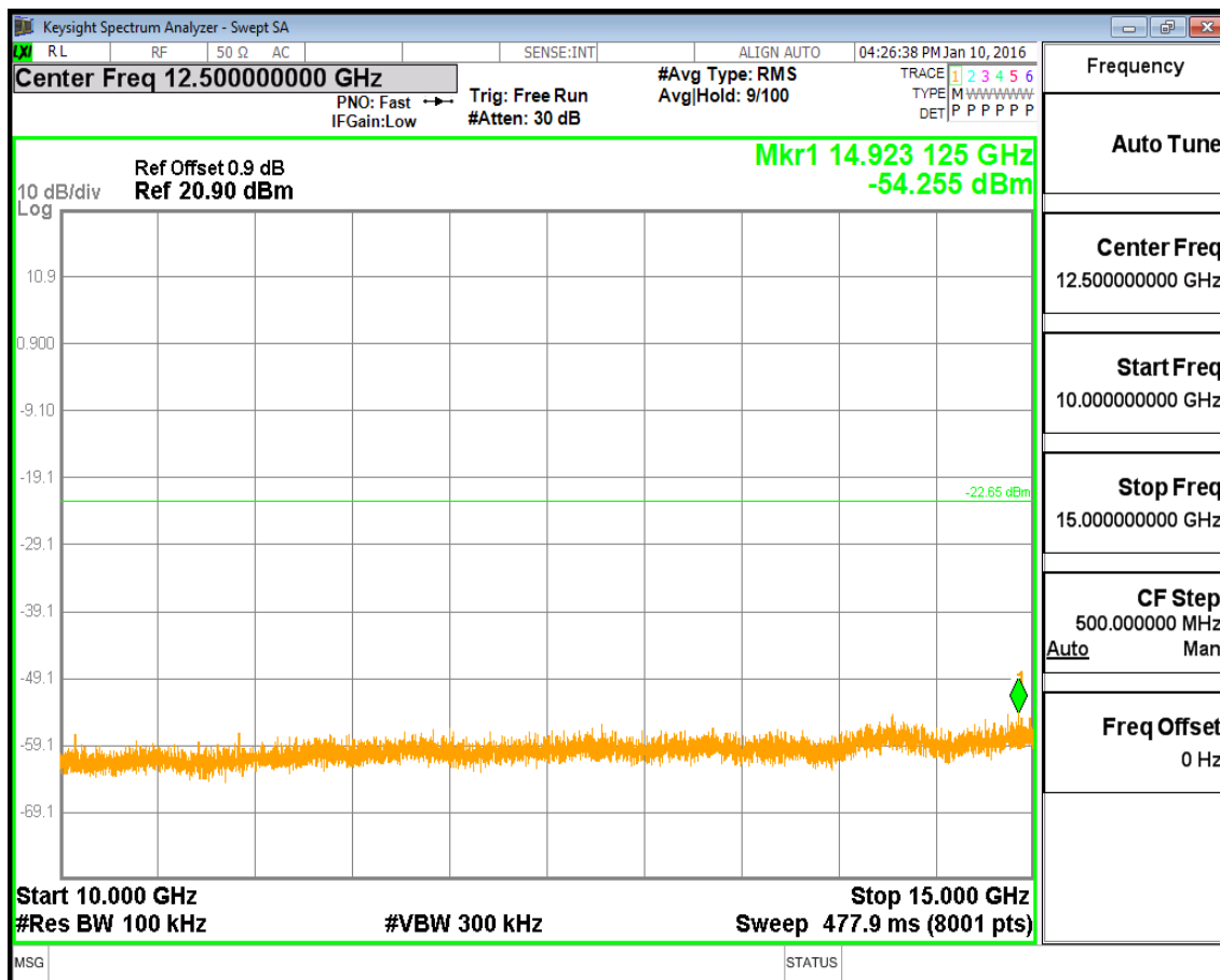
(Plot 4.5.1 A5: Channel 00: 2402MHz @ GFSK)
