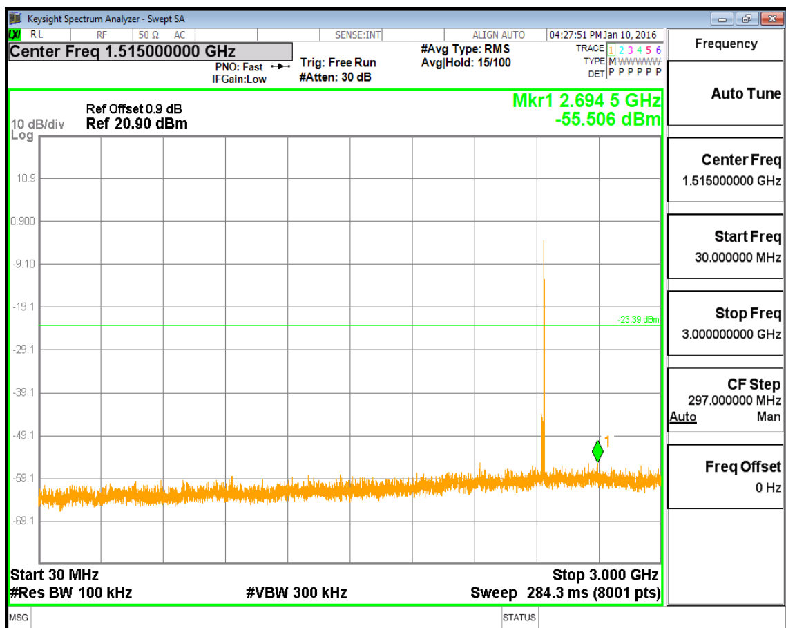
(Plot 4.5.1 B2: Channel 19: 2440MHz @ GFSK)
