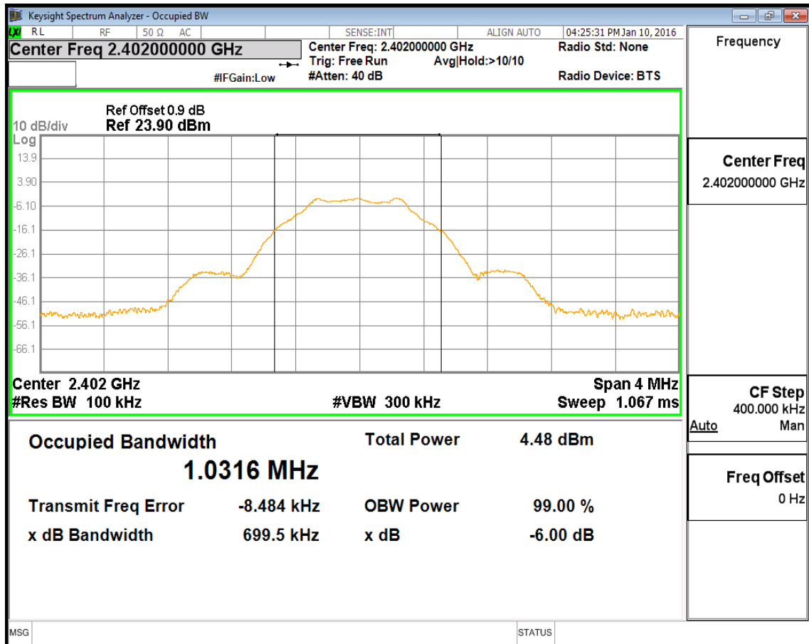
(Plot 4.6.1 A: Channel 00: 2402MHz @ GFSK)
