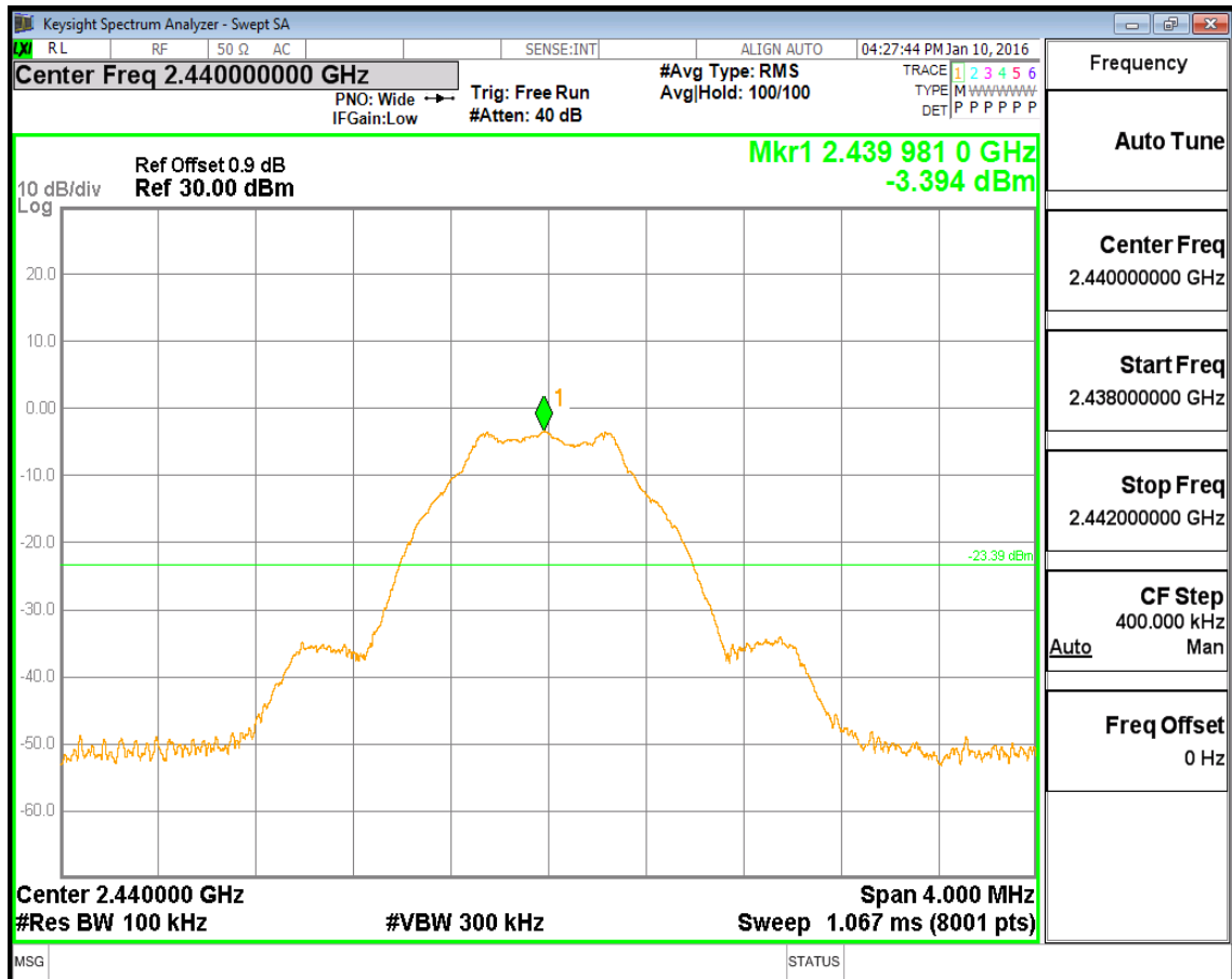
(Plot 4.5.1 B1: Channel 19: 2440MHz @ GFSK)
