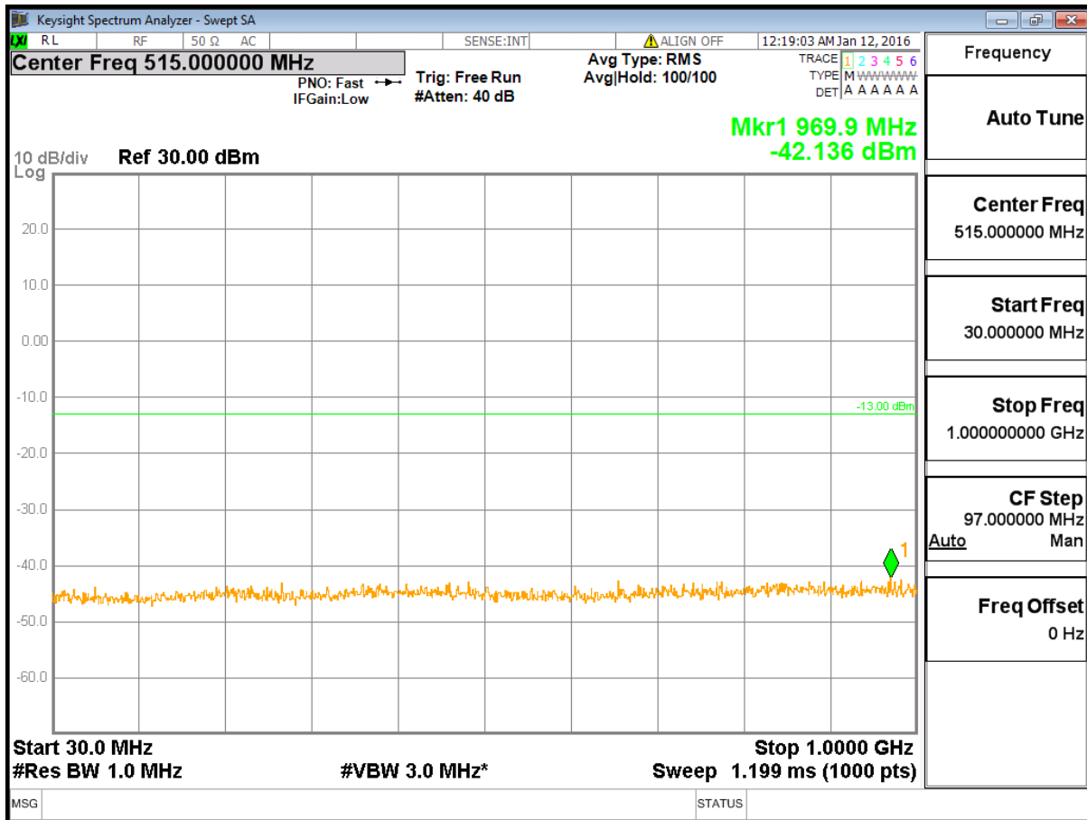
4.5.2 B3: Channel 661: 1880.00MHz @ Traffic @ PCS1900)
