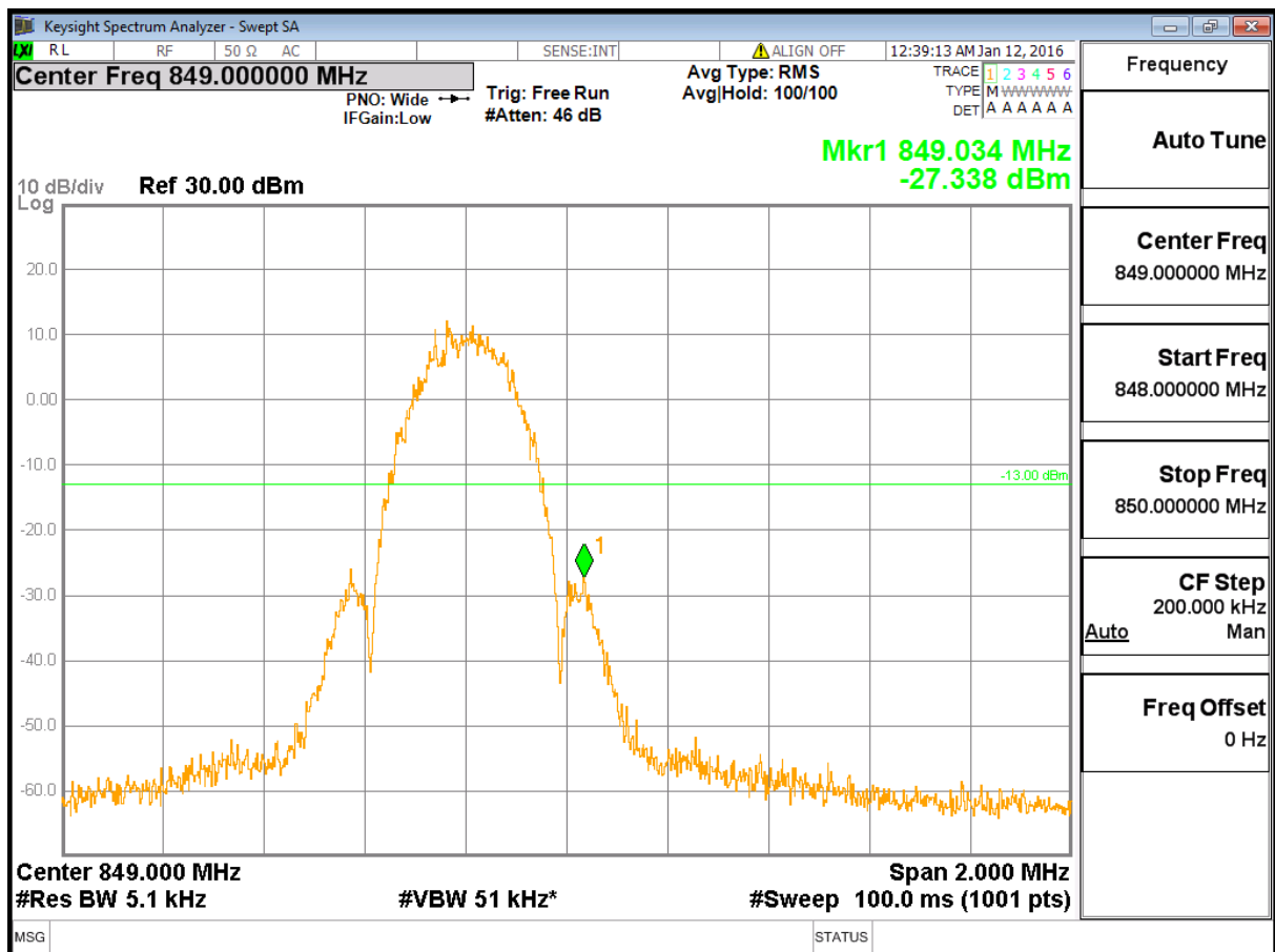
(Plot 4.4.2 B: Channel 251: 848.80MHz @ EGPRS850)
