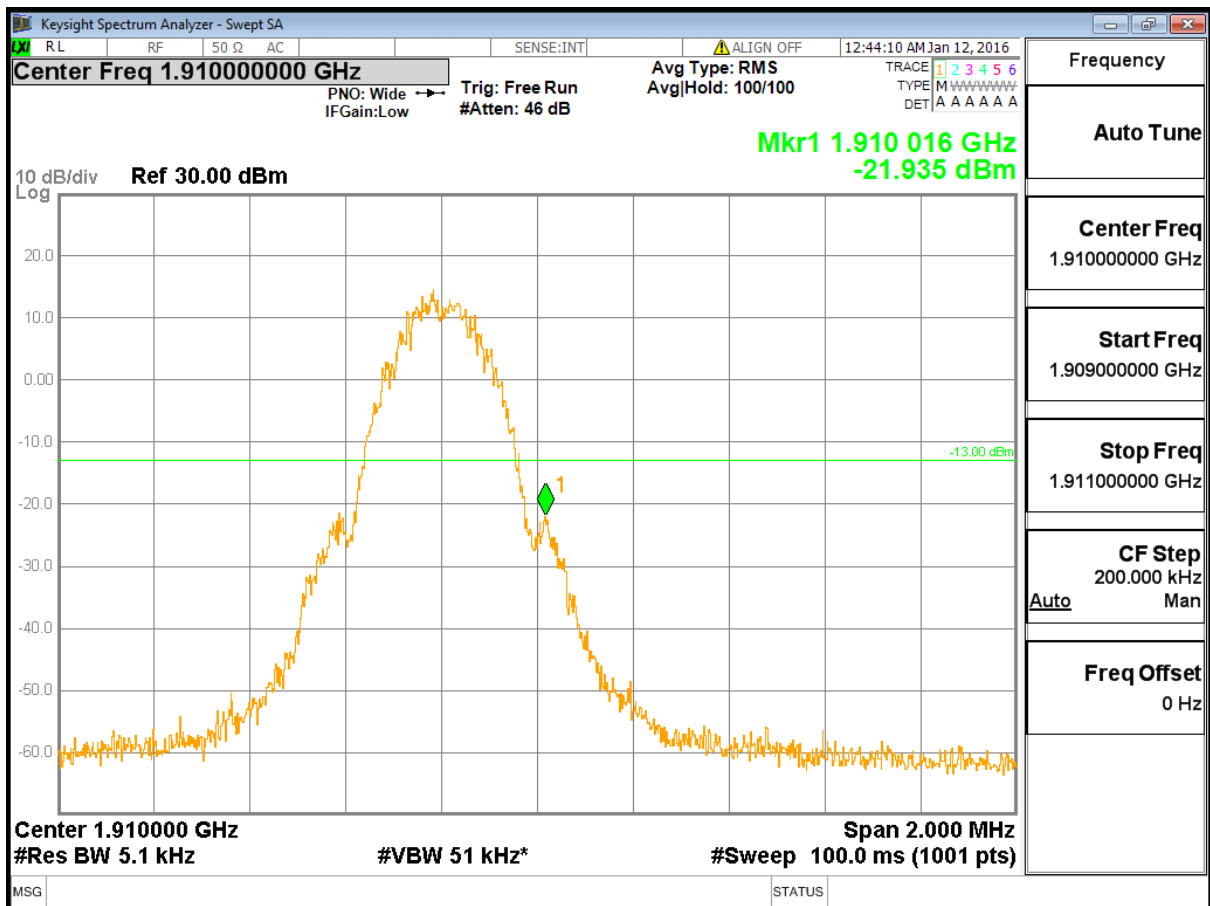
4.4.3 B: Channel 810: 1909.80MHz @ PCS1900)
