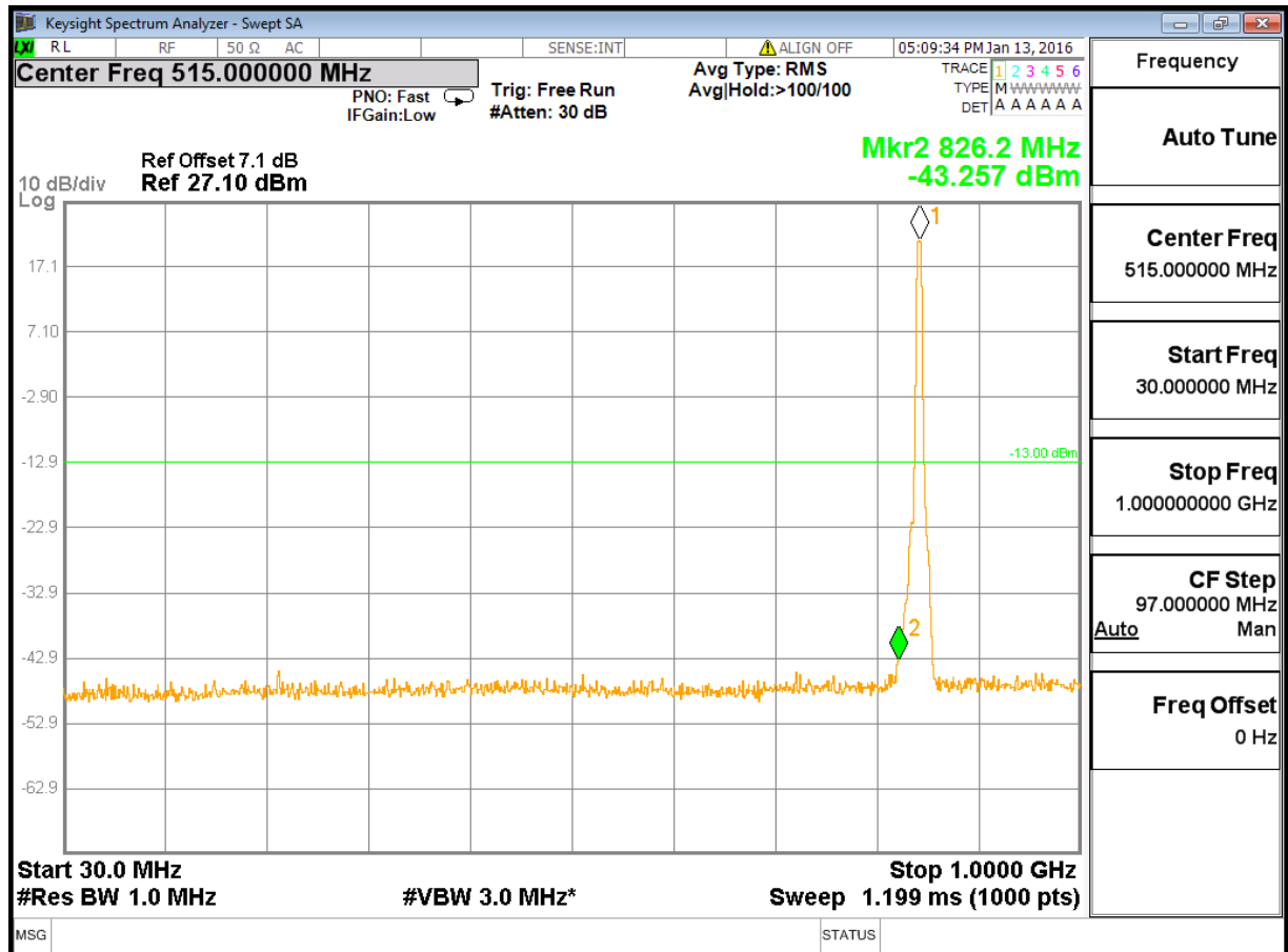
(Plot 4.5.2 C3: Channel 4233: 846.60 MHz @ WCDMA Band V)
