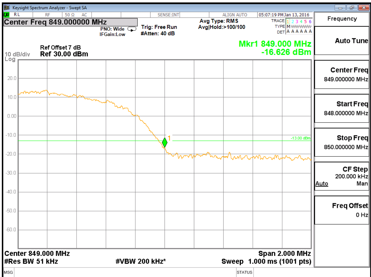
(Plot 4.5.2 B: Channel 4233: 846.6MHz @ WCDMA Band V)
