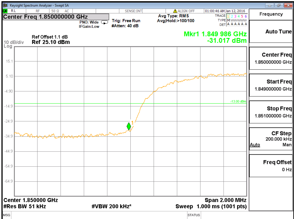
(Plot 4.5.1 A: Channel 9262: 1852.4MHz WCDMA Band II)
