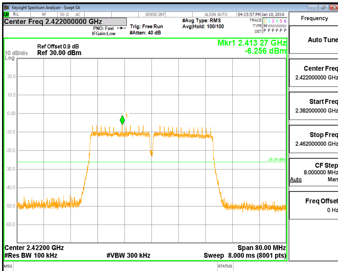
(Plot 4.5.4 A1: Channel 3: 2422MHz @ 802.11n HT40)
