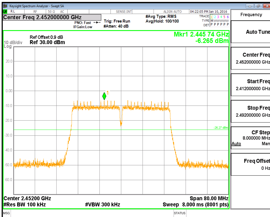
(Plot 4.5.4 C1: Channel 9 : 2452MHz @ 802.11n HT40)
