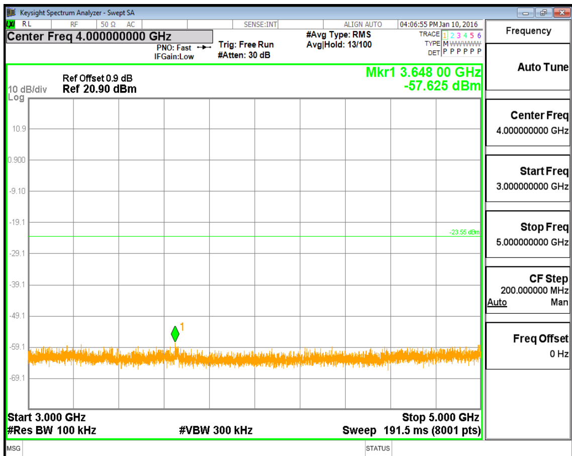
(Plot 4.5.2 B3: Channel 6: 2437MHz @ 802.11g)
