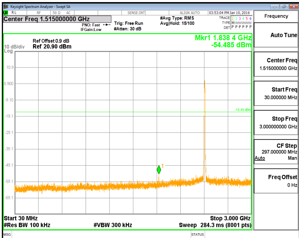
(Plot 4.5.1 A2: Channel 1: 2412MHz @ 802.11b)
