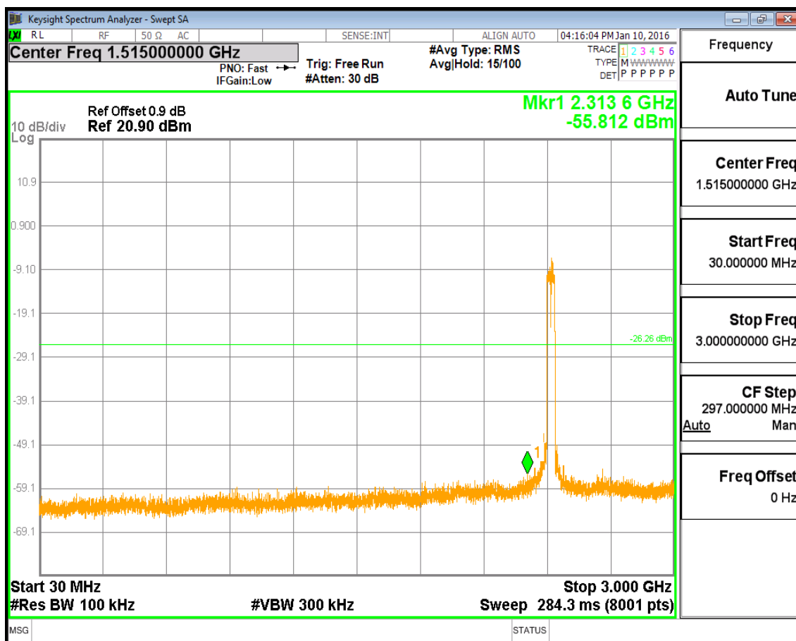
(Plot 4.5.4 A2: Channel 3: 2422MHz @ 802.11n HT40)
