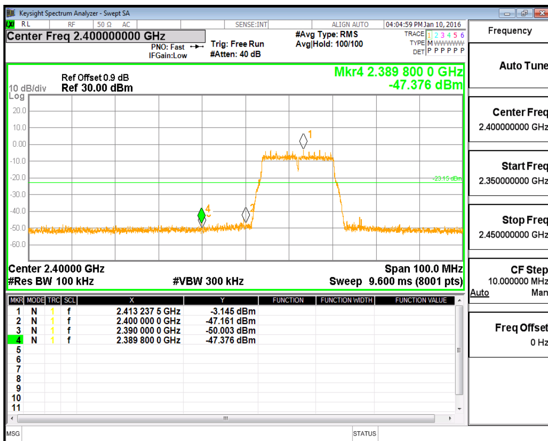
(Plot 4.5.2 D1: Left Band edge @ 802.11g)
