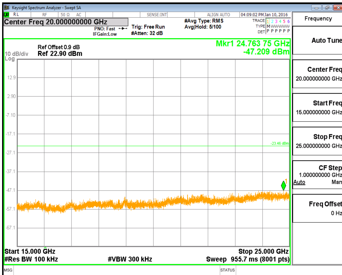
(Plot 4.5.2 C6: Channel 11: 2462MHz @ 802.11g)
