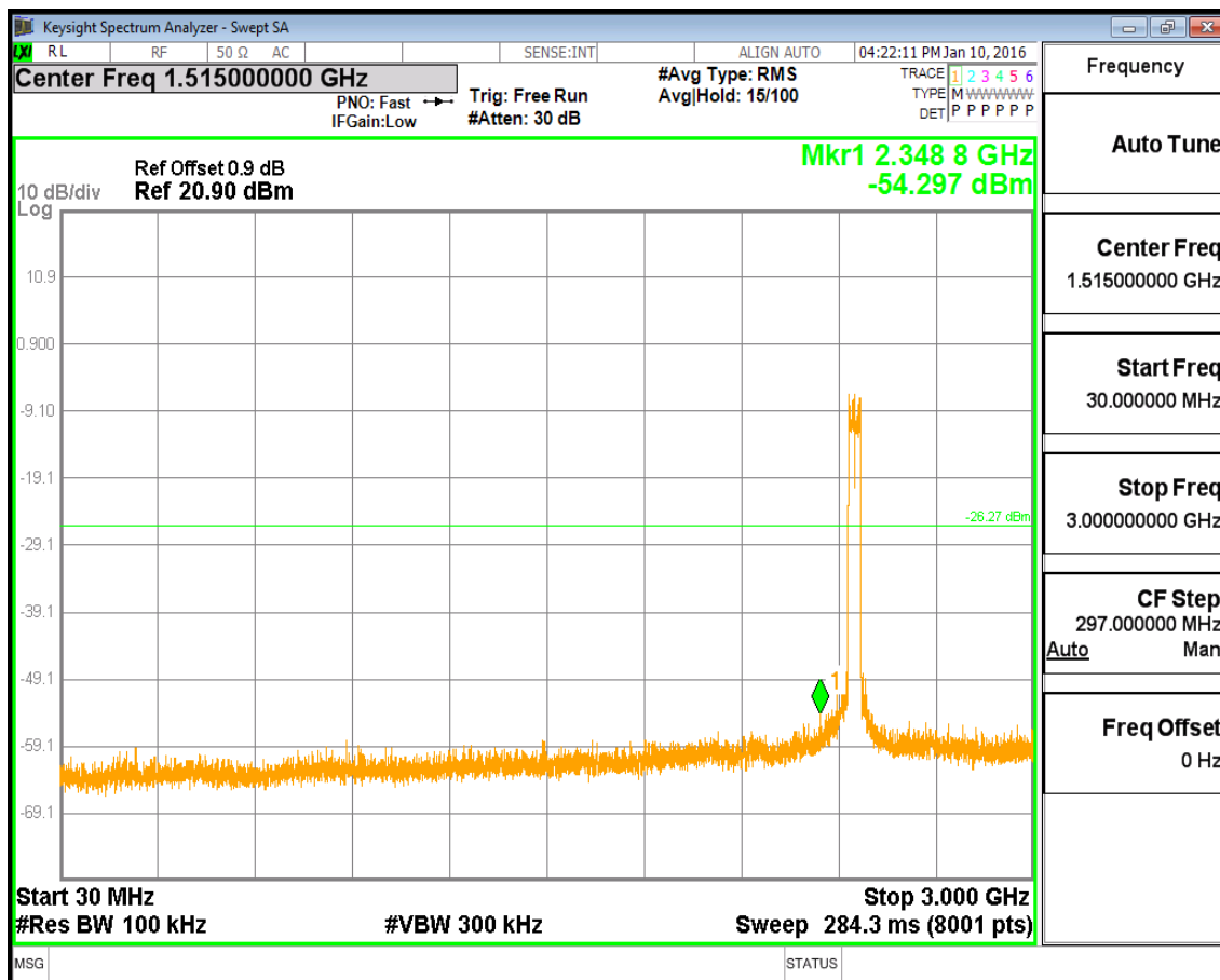
(Plot 4.5.4 C2: Channel 9: 2452MHz @ 802.11n HT40)
