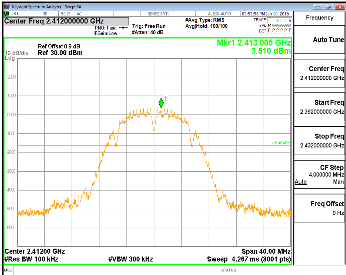
(Plot 4.5.1 A1: Channel 1: 2412MHz @ 802.11b)
