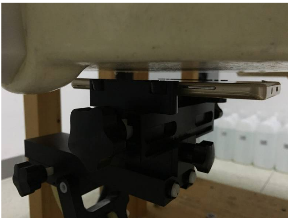
10mm Front Side Setup Photo
