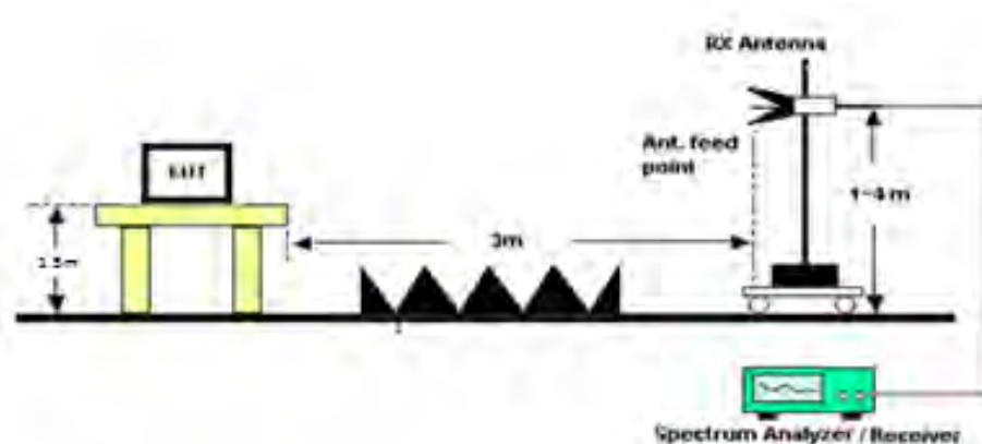
Radiated Measurement
