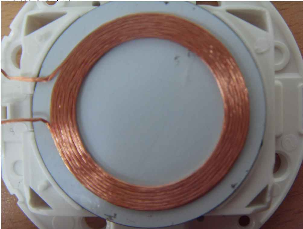
Antenna_Wireless Charging
