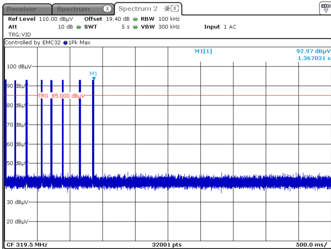
Figure 8.4-1: Transmission duration after activation (within 5 seconds)
