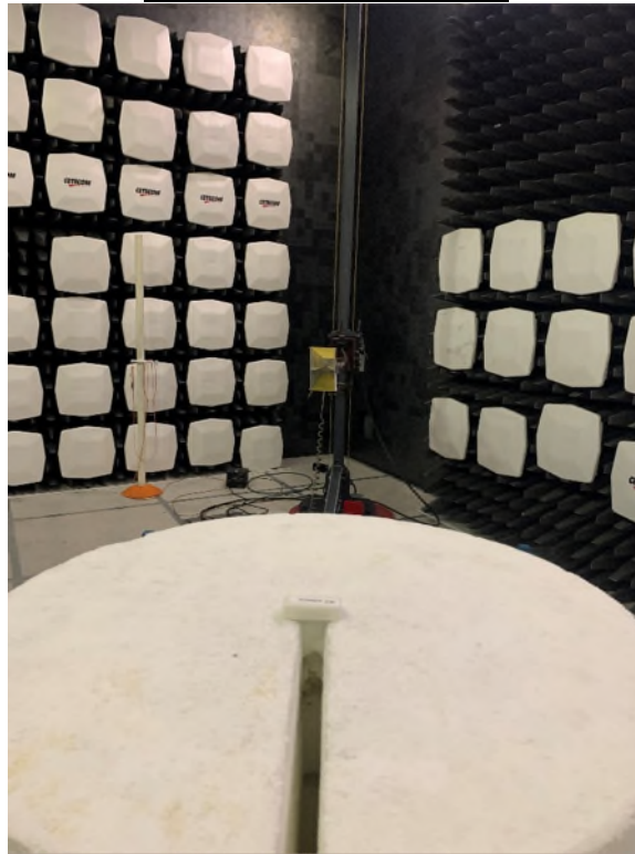
1 GHz to 3 GHz Rear View
