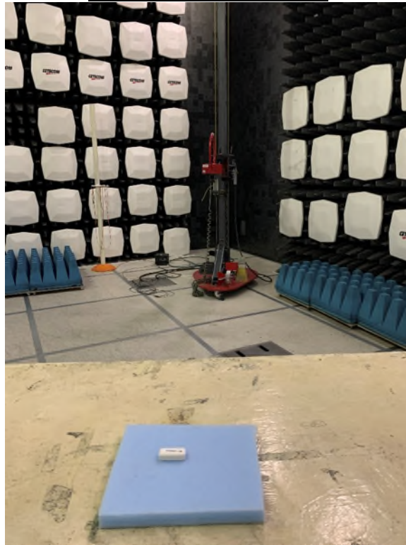
9 kHz to 30 MHz Front View
