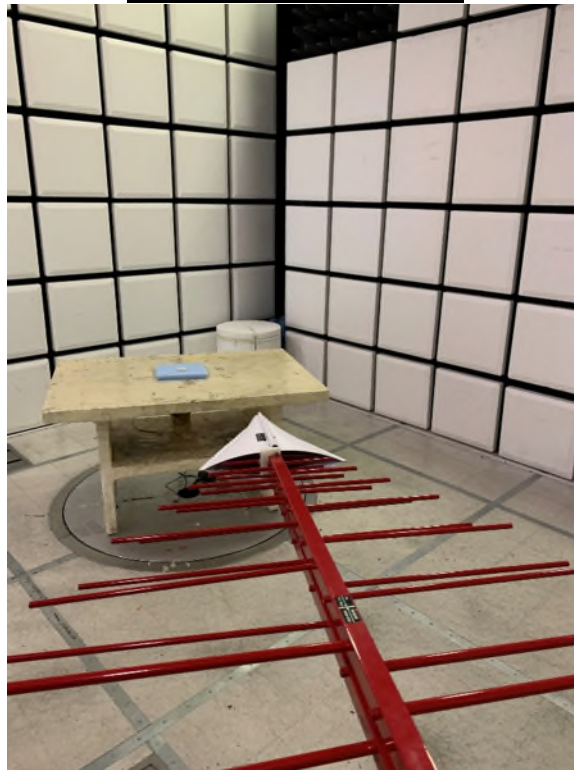
30 MHz to 1 GHz Rear View
