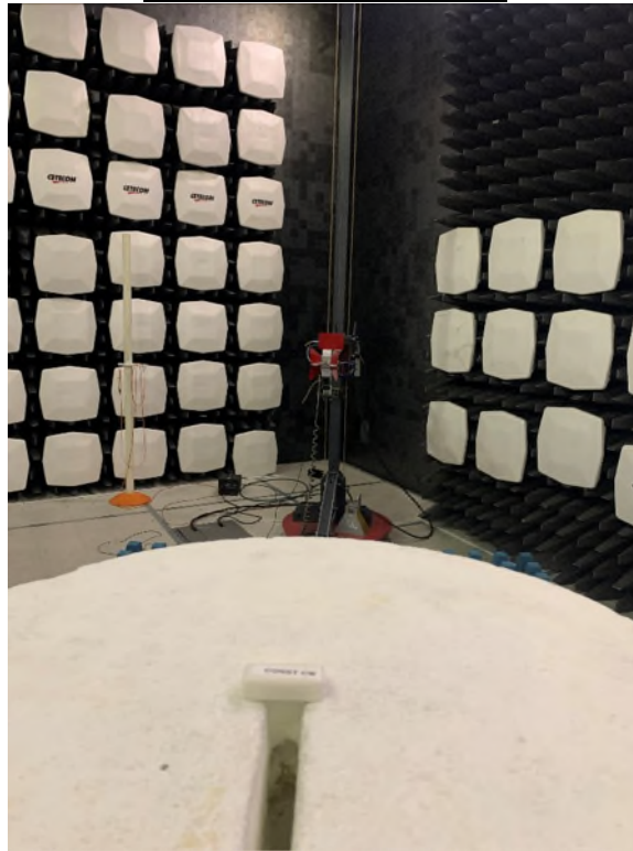
3 GHz to 4 GHz Rear View
