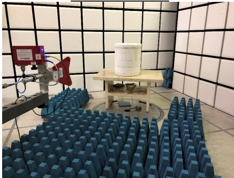
3 GHz to 4 GHz Rear View
