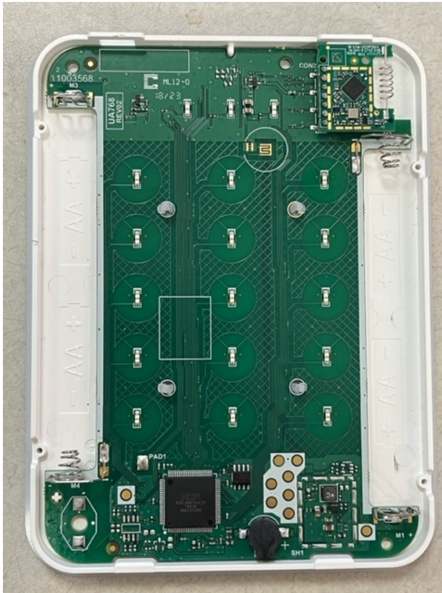
IQ Keypad-PG top side of PCB assembly (UA768 + RF module)
