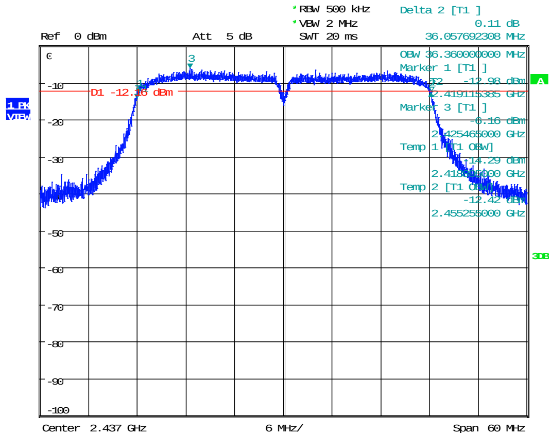
Plot 1.20 – 99% Bandwidth
