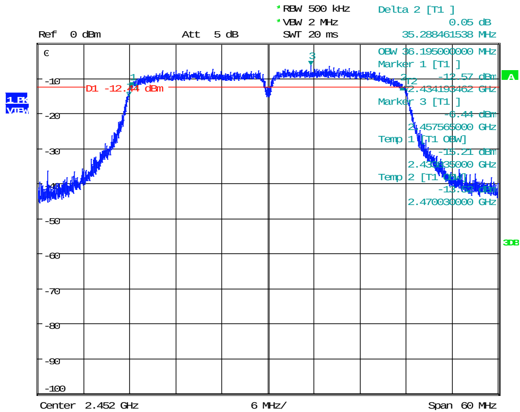
Plot 1.21 – 99% Bandwidth
