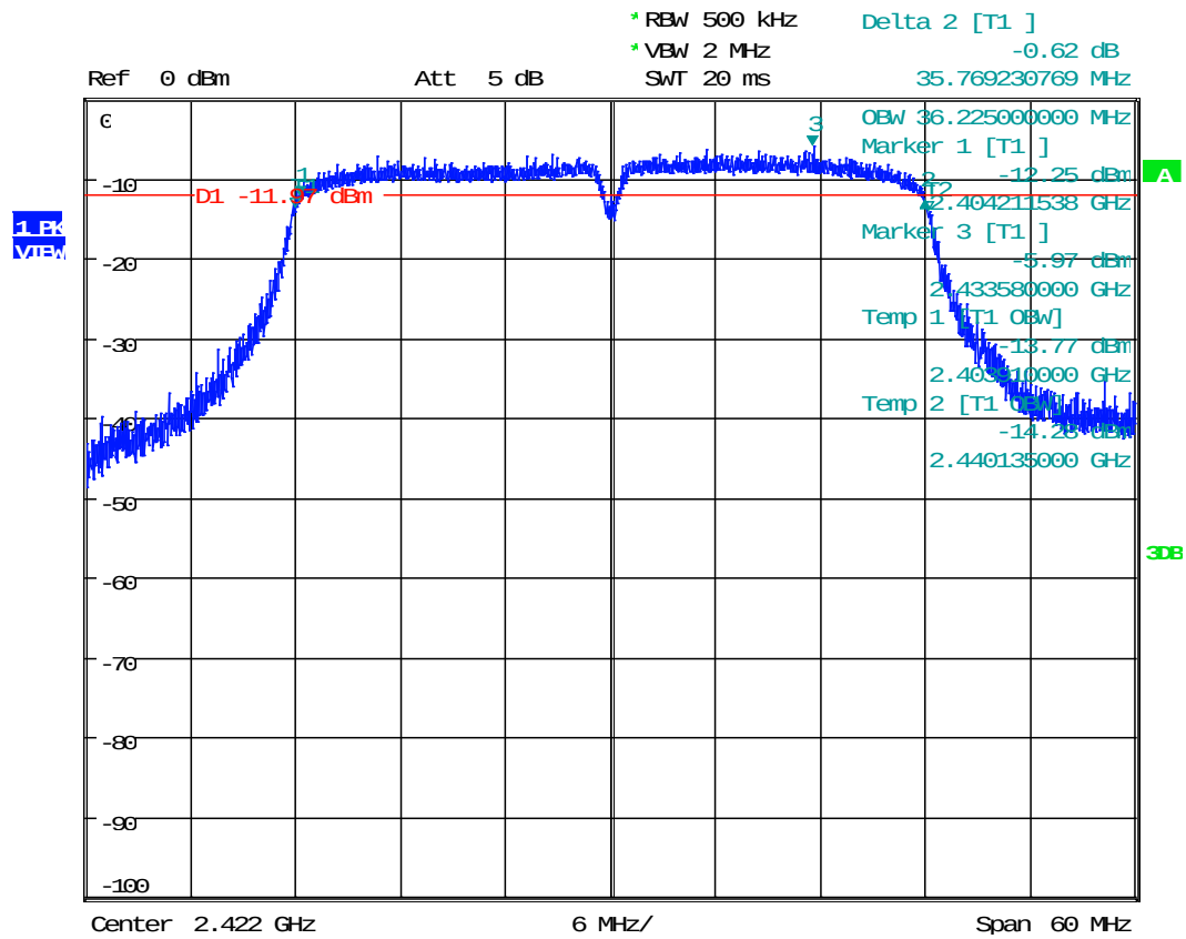
Plot 1.19 – 99% Bandwidth
