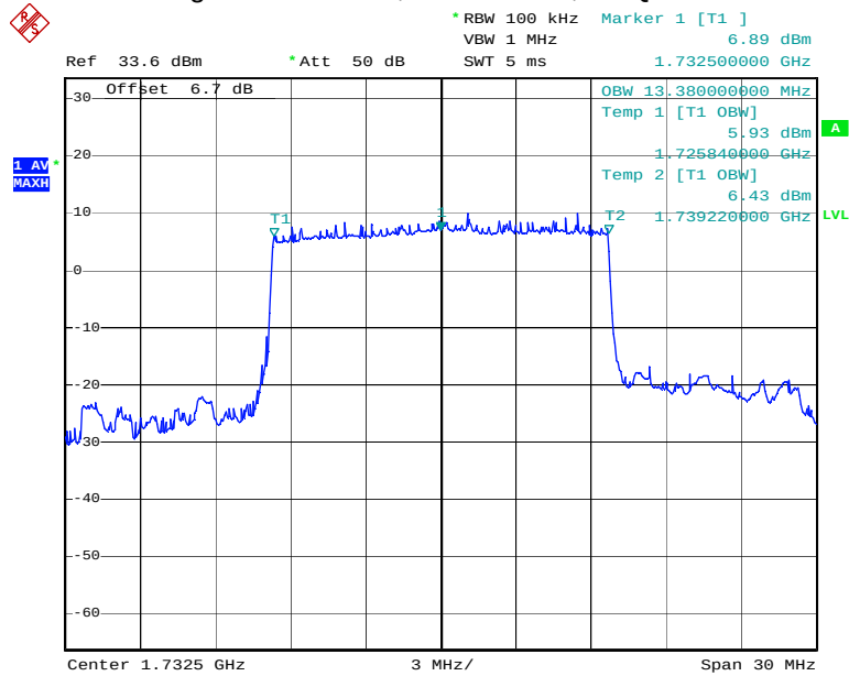
Figure 14: Band 4, BW=15MHz, 16-QAM
