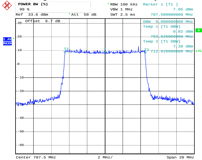
Figure 24: Band 12, BW=10MHz, 16-QAM
