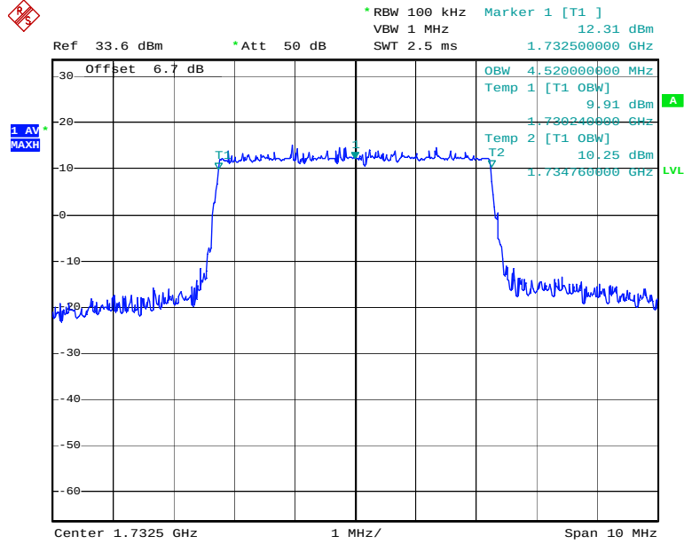
Figure 9: Band 4, BW=5MHz, QPSK
