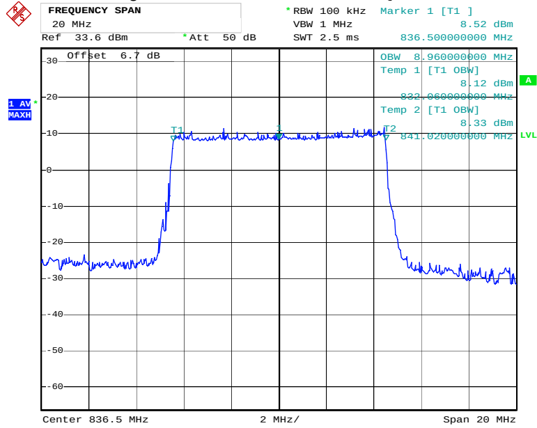
Figure 19: Band 5, BW=10MHz, QPSK
