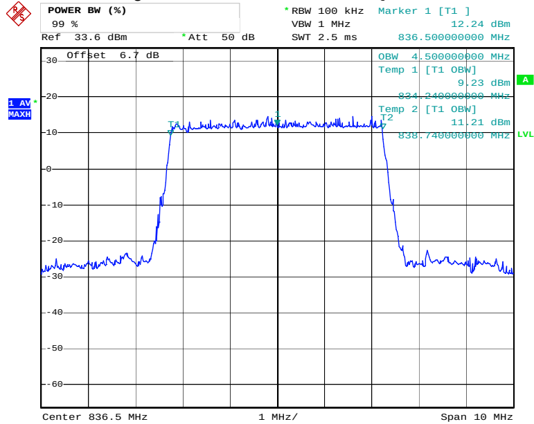
Figure 17: Band 5, BW=5MHz, QPSK
