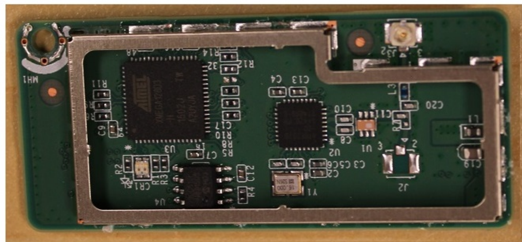
Top view, shield rib removed
