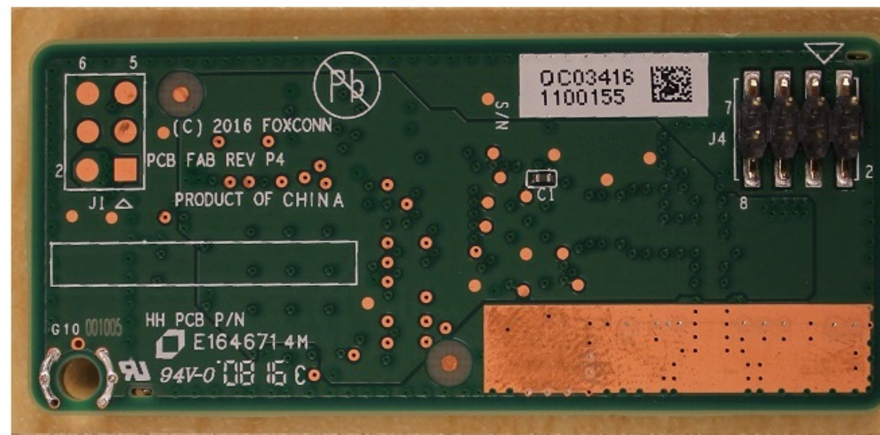
Bottom view
