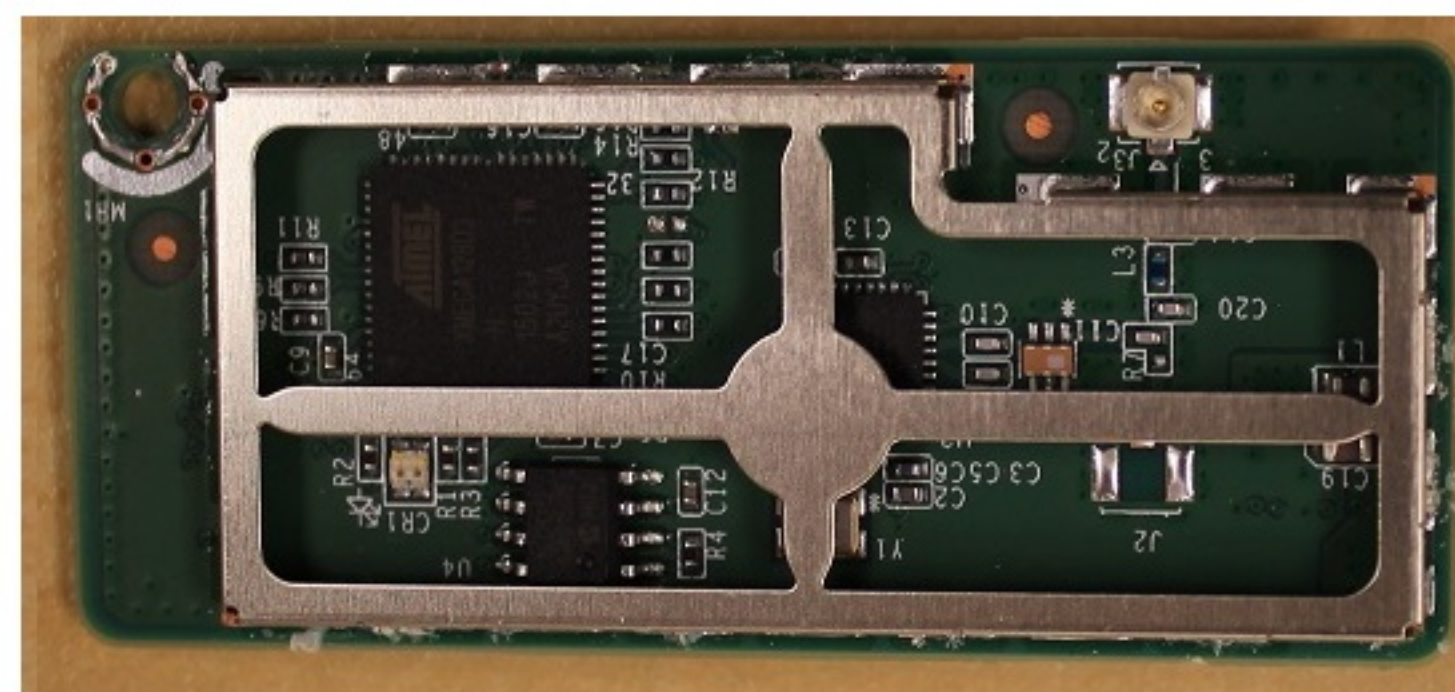
Top View, Shield top removed
