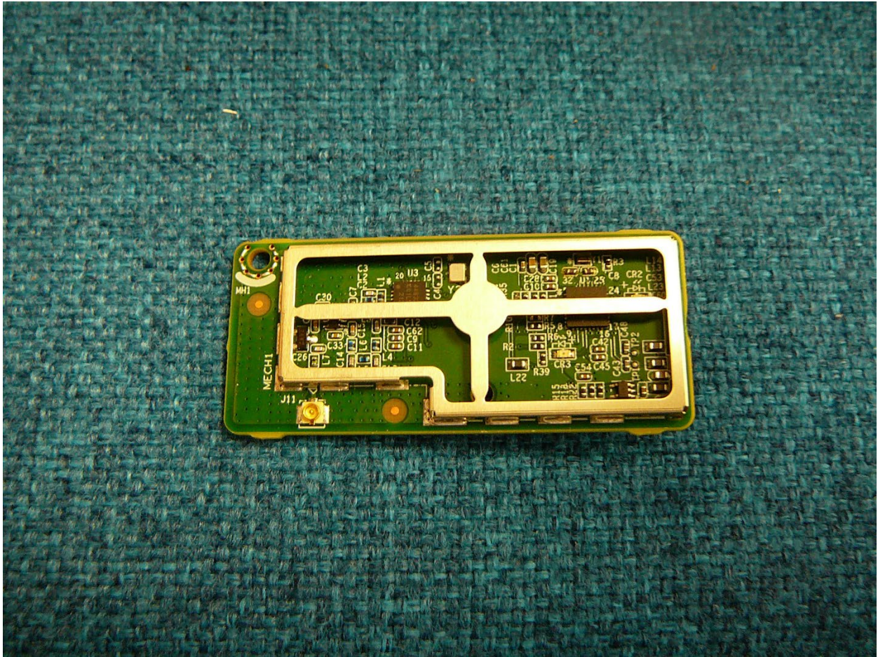
SRF319H – Top View with Cover Removed
