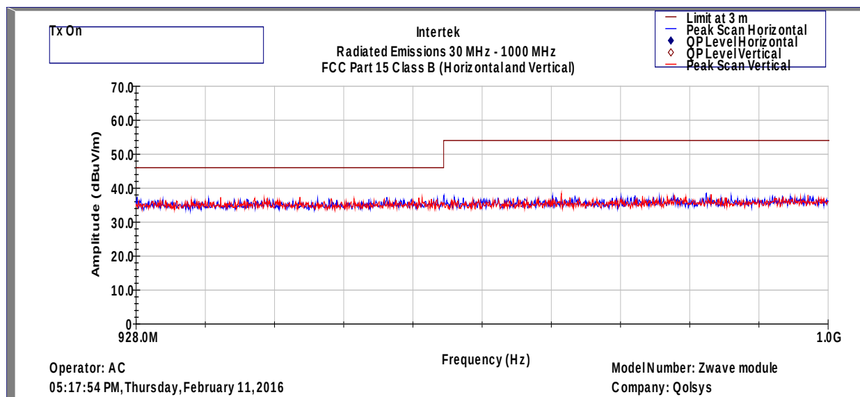
Plot 2: Spurious Emissions, 928MHz to 1000MHz, Peak
