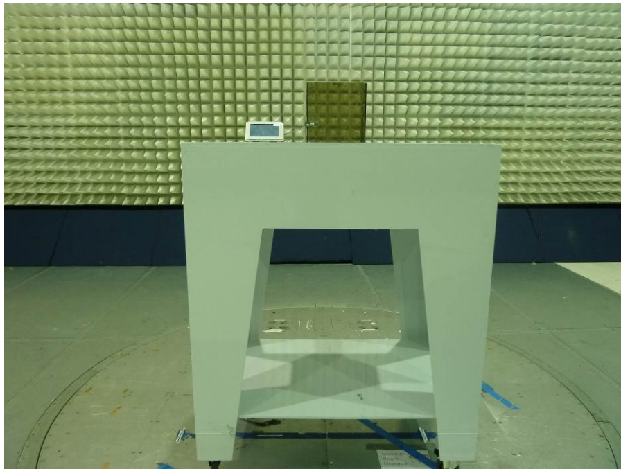
Radiated Emissions
