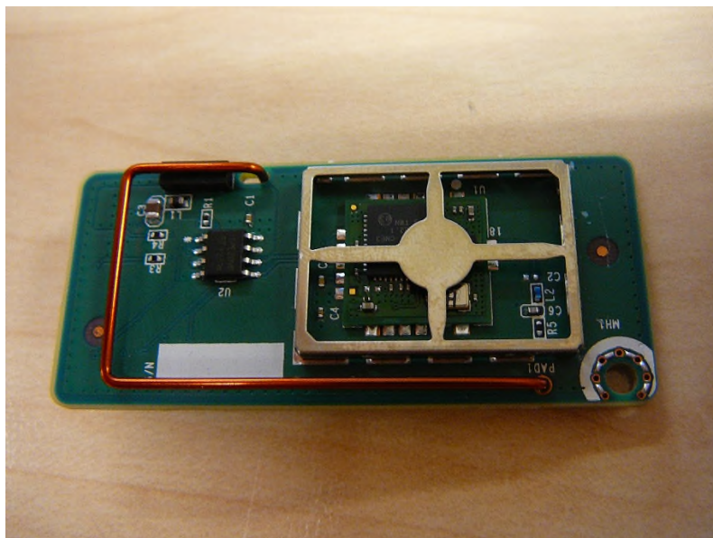
QS-ZwaveAH – Top View with Cover Removed
