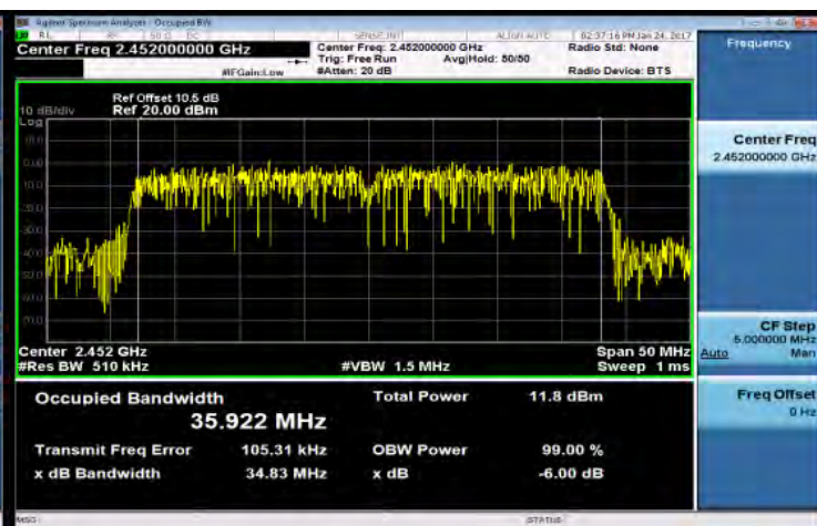
99% BW 802.11n_HT40M CH-High
