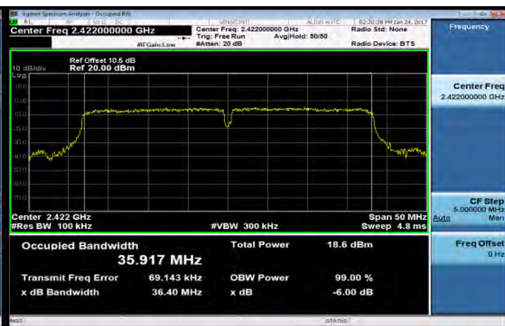
6dB BW 802.11n_HT40M CH-Mid
