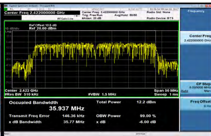
99% BW 802.11n_HT40M CH-Mid
