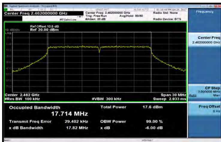
6dB BW 802.11n_HT20M CH-High
