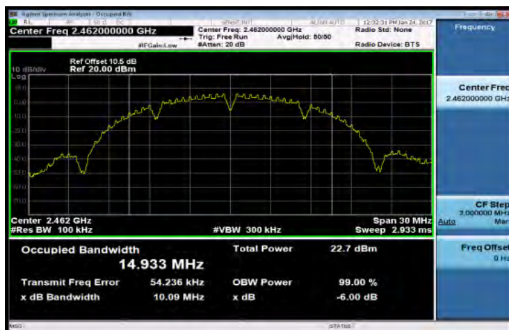
6dB BW 802.11b CH-High
