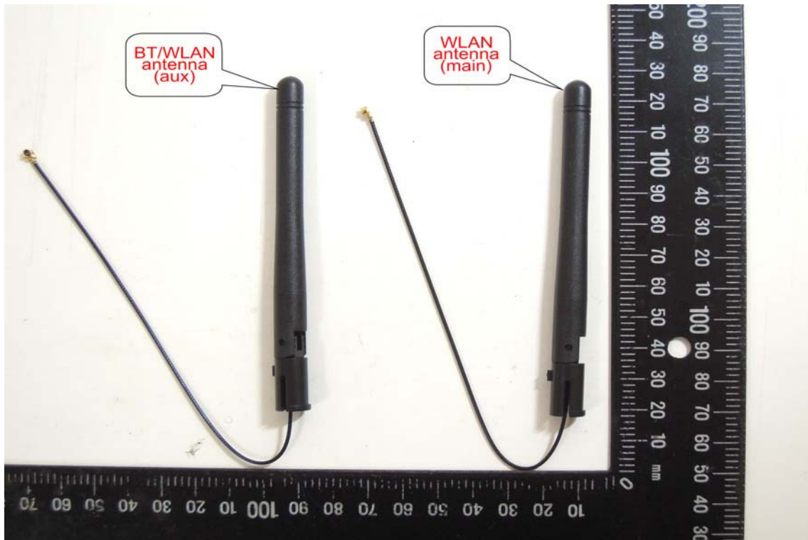
Antenna #2
