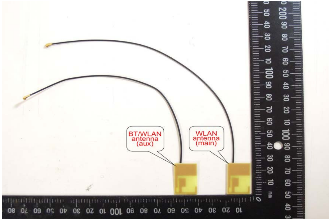
Antenna #2
